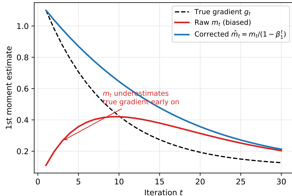
Adam: Bias Correction of 1st Moment ( \beta_1 = 0.9 )
