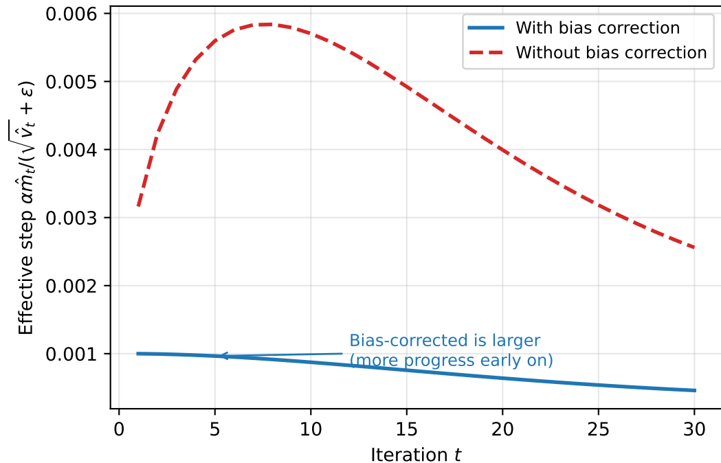
Adam: Effective Update Magnitude ( \alpha = 0.001 )
