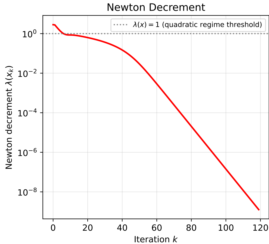
Newton Convergence Phases on Rosenbrock (120 iterations, \alpha = 0.22 )
