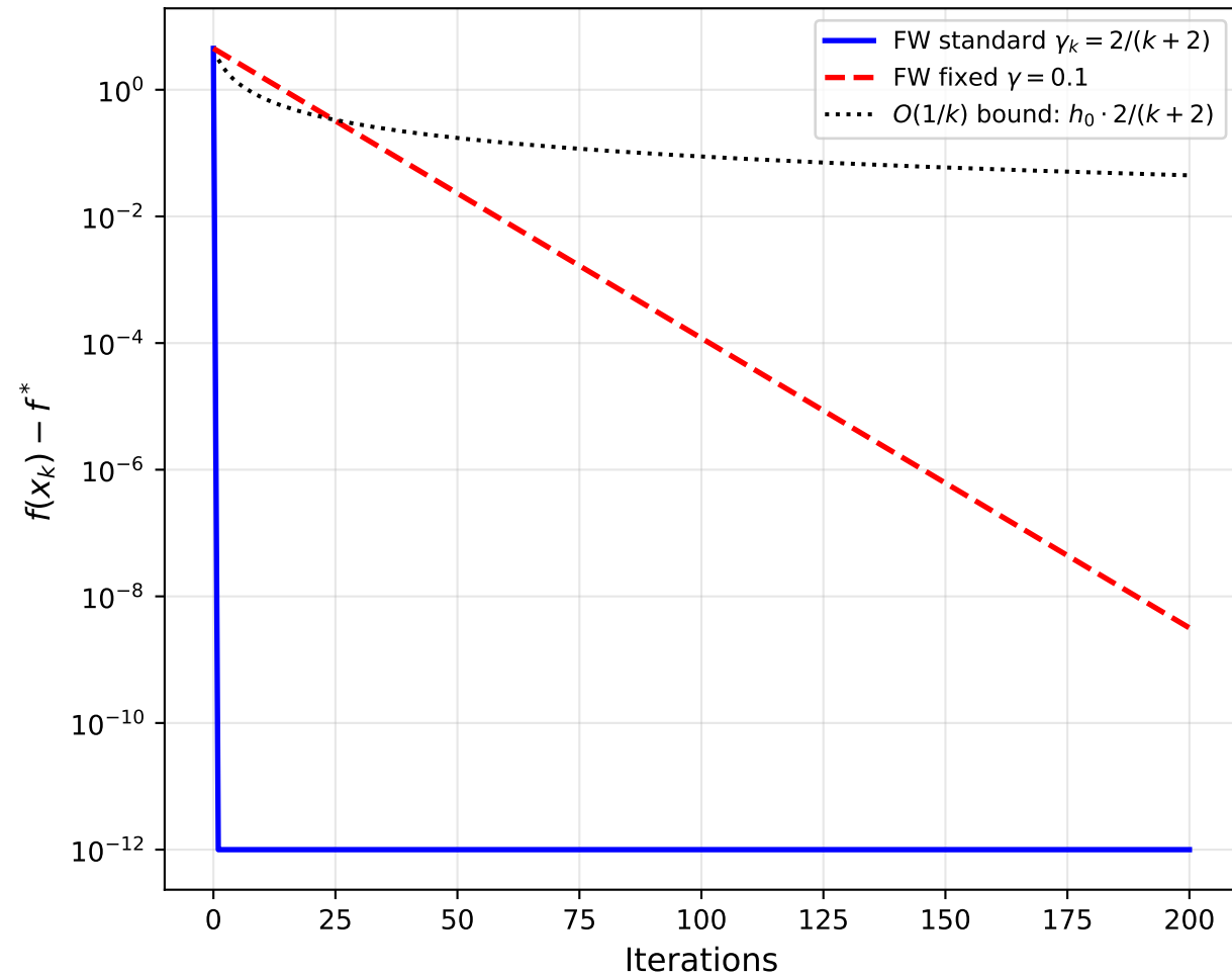
FW Rate Tightness: O(1/k) on Linear Program (Simplex)
