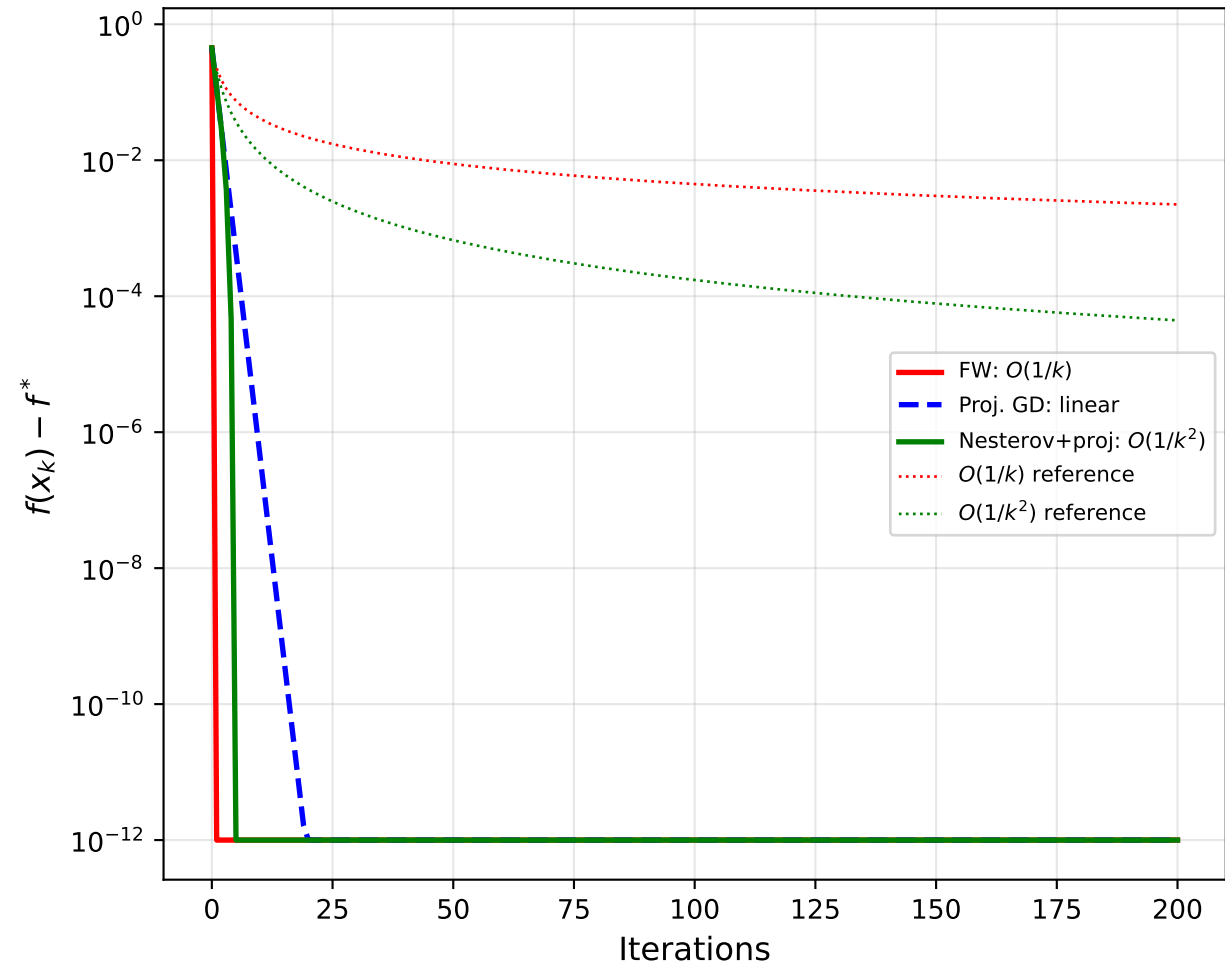
FW vs. Proj. GD vs. FISTA on Quadratic Over Simplex
