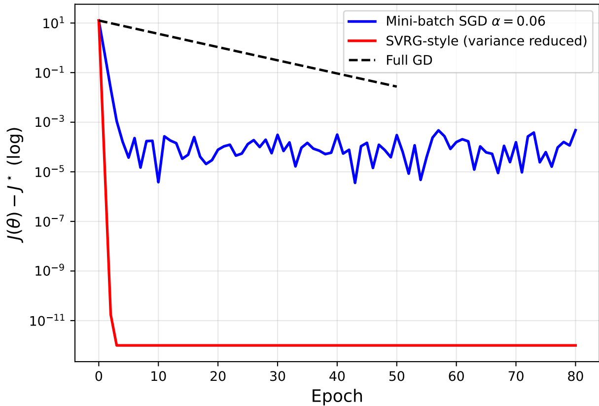
Variance Reduction: SGD vs SVRG-style
