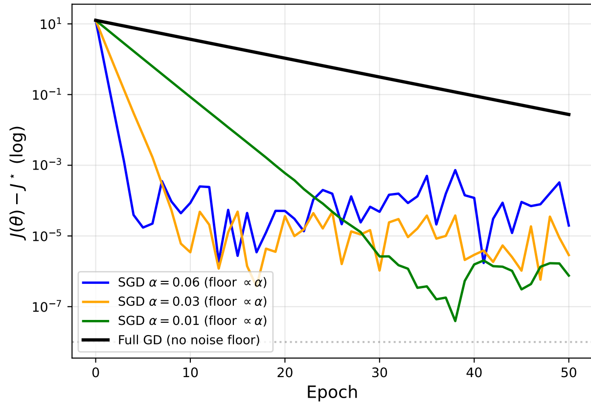
SGD Noise Floor vs Step Size (batch size b = 40 )
