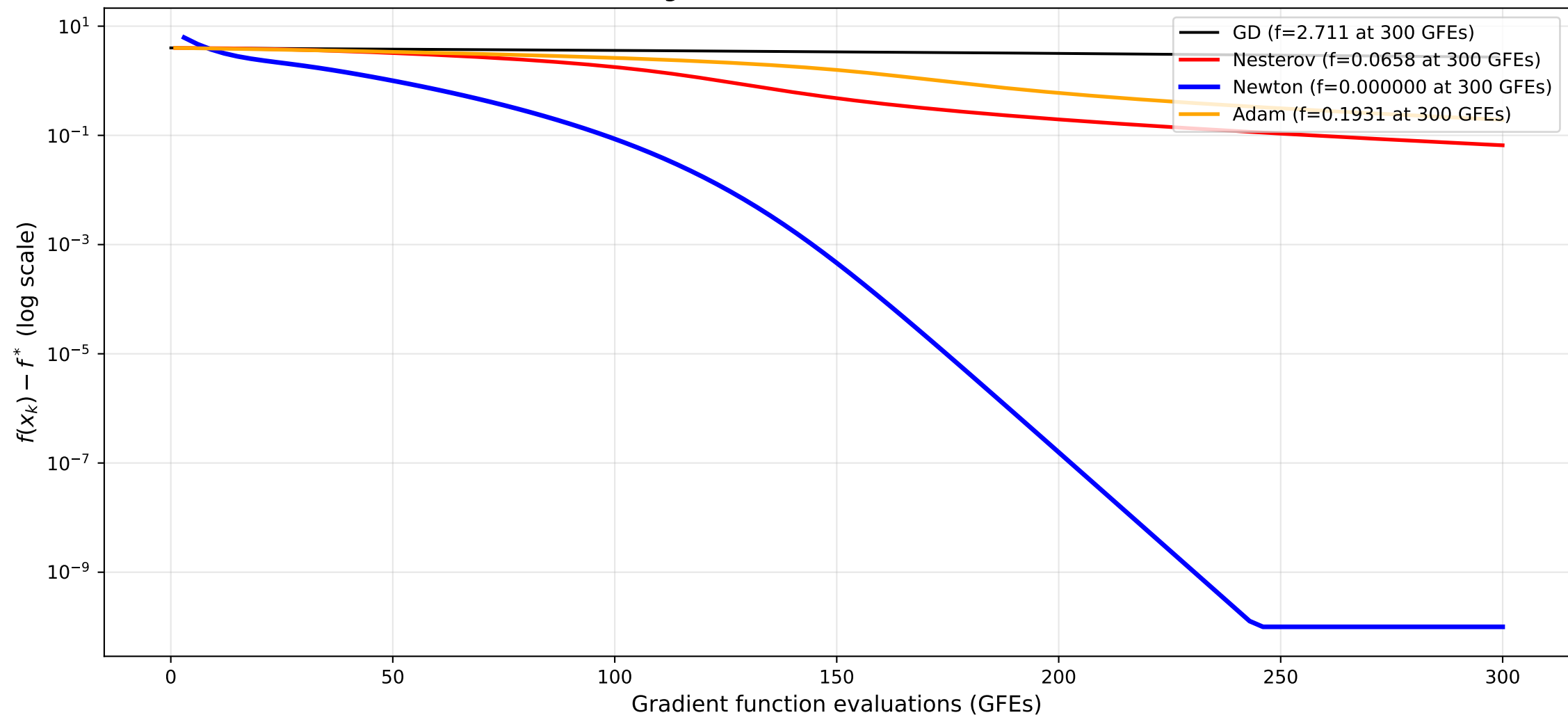
Fair Comparison: Benchmark C at Equal Gradient Evaluation Budget (300 GFEs) Newton: 3 GFEs/iter (gradient + Hessian); GD/Nesterov/Adam: 1 GFE/iter
