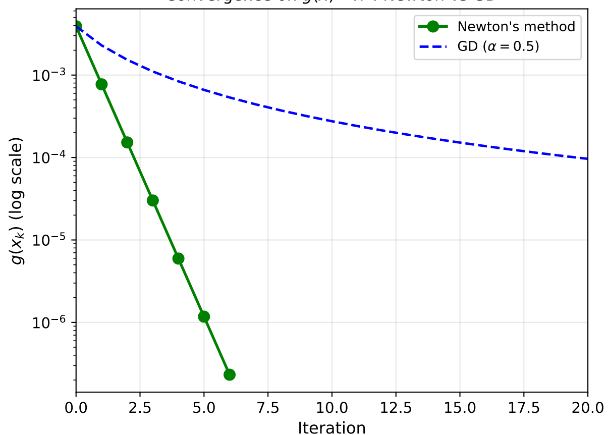
Convergence on g(x) = x^4 : Newton vs GD
