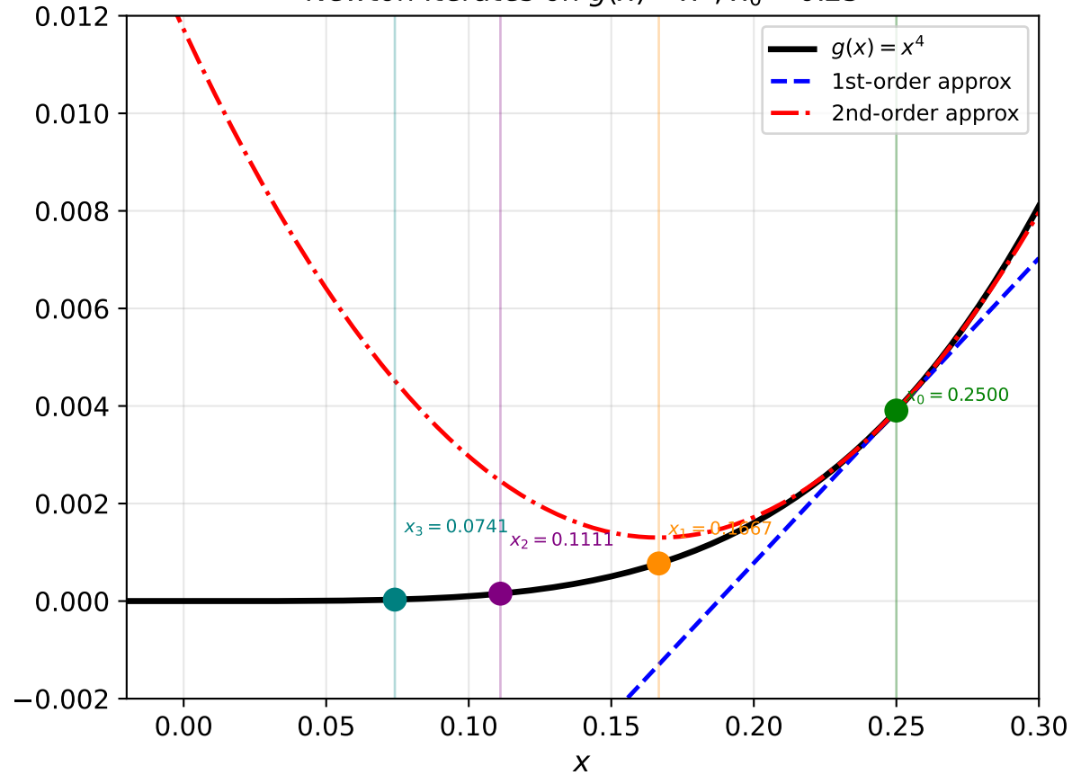
Newton Iterates on g(x) = x^4 , x_0 = 0.25
