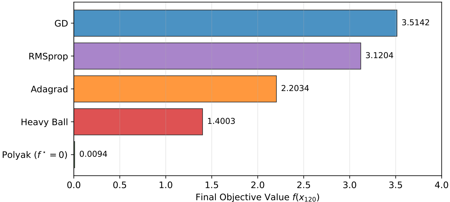
Q1: Method Ranking on Rosenbrock (Benchmark C, 120 iterations)
