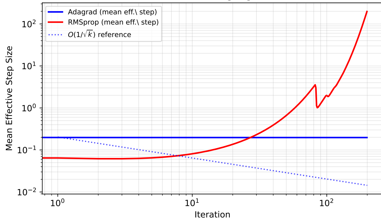
Adagrad vs RMSprop: Step-Size Decay (Benchmark B, log-log scale)
