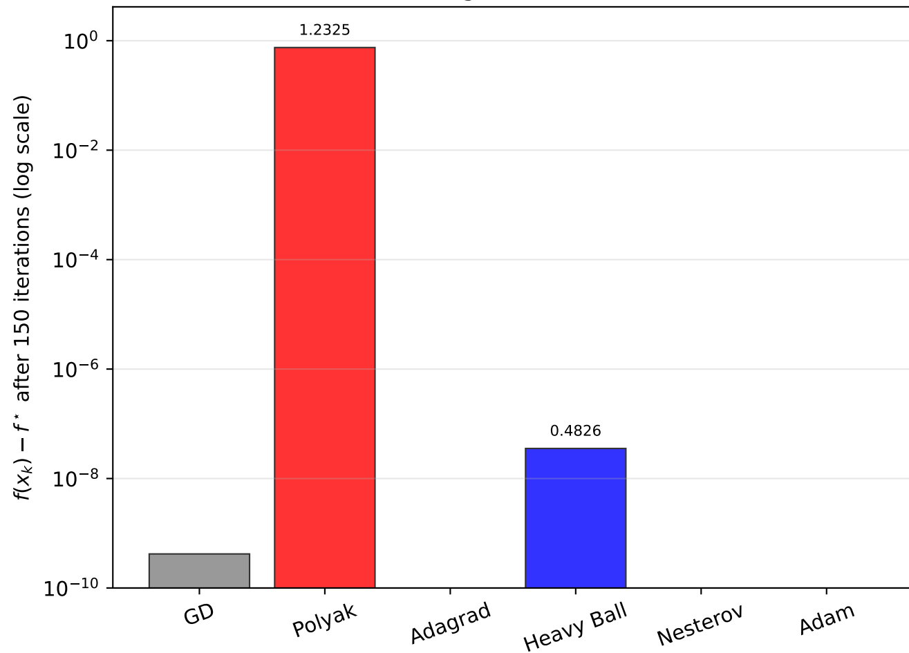
Benchmark A: Final Convergence Gap (Linear Regression, \kappa \approx 1.12 )
