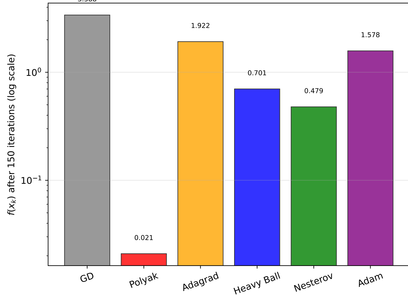
Benchmark C: Final Objective (Rosenbrock, \kappa \approx 2508 )
