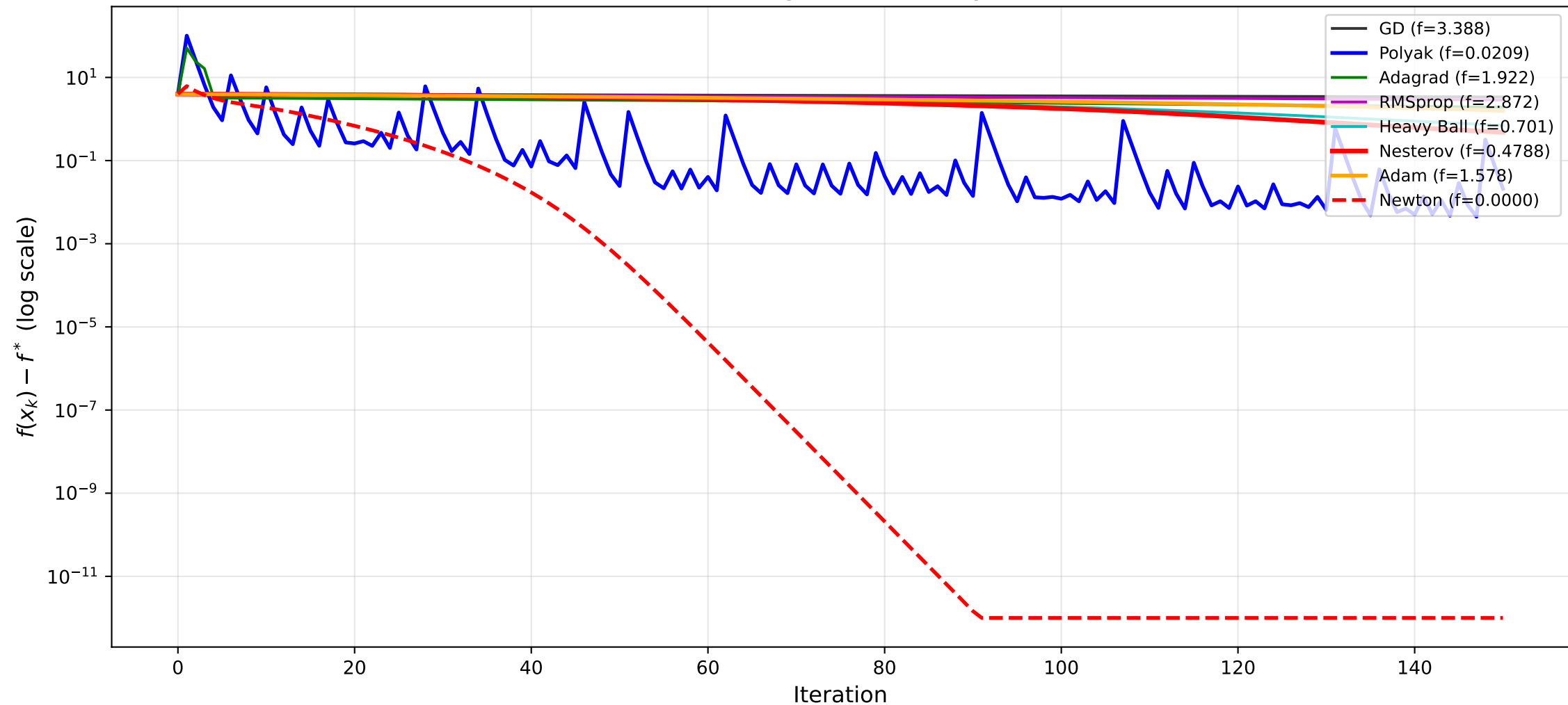
All Methods on Benchmark C (Rosenbrock, \kappa \approx 2508 ): 150 Iterations Convergence Hierarchy
