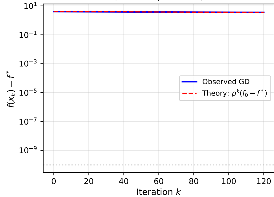
Benchmark C ( \kappa \approx 2508 , \rho \approx 0.9992 )
