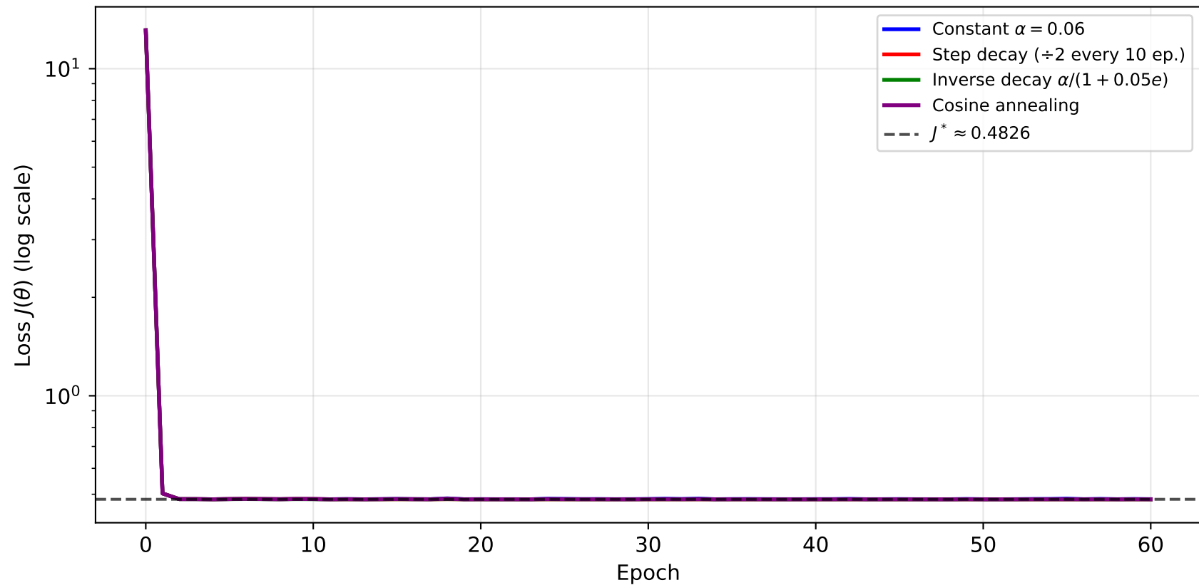
Q2: Mini-Batch SGD ( b = 20 ) with Different Learning Rate Schedules (Benchmark A)
