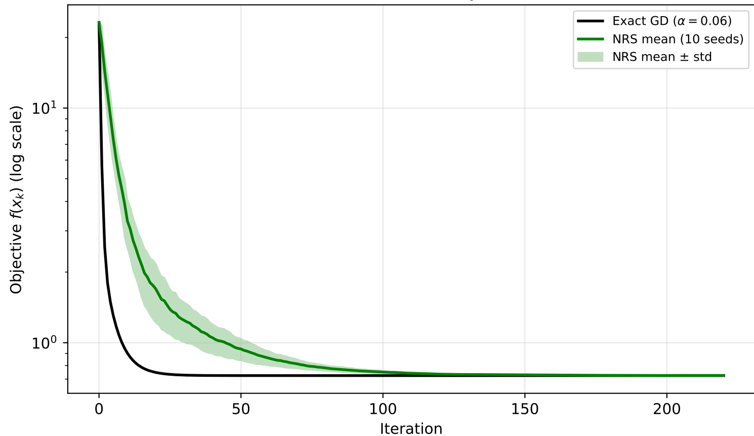
Q4A: Nesterov Random Search Variability (10 seeds, Benchmark B)
