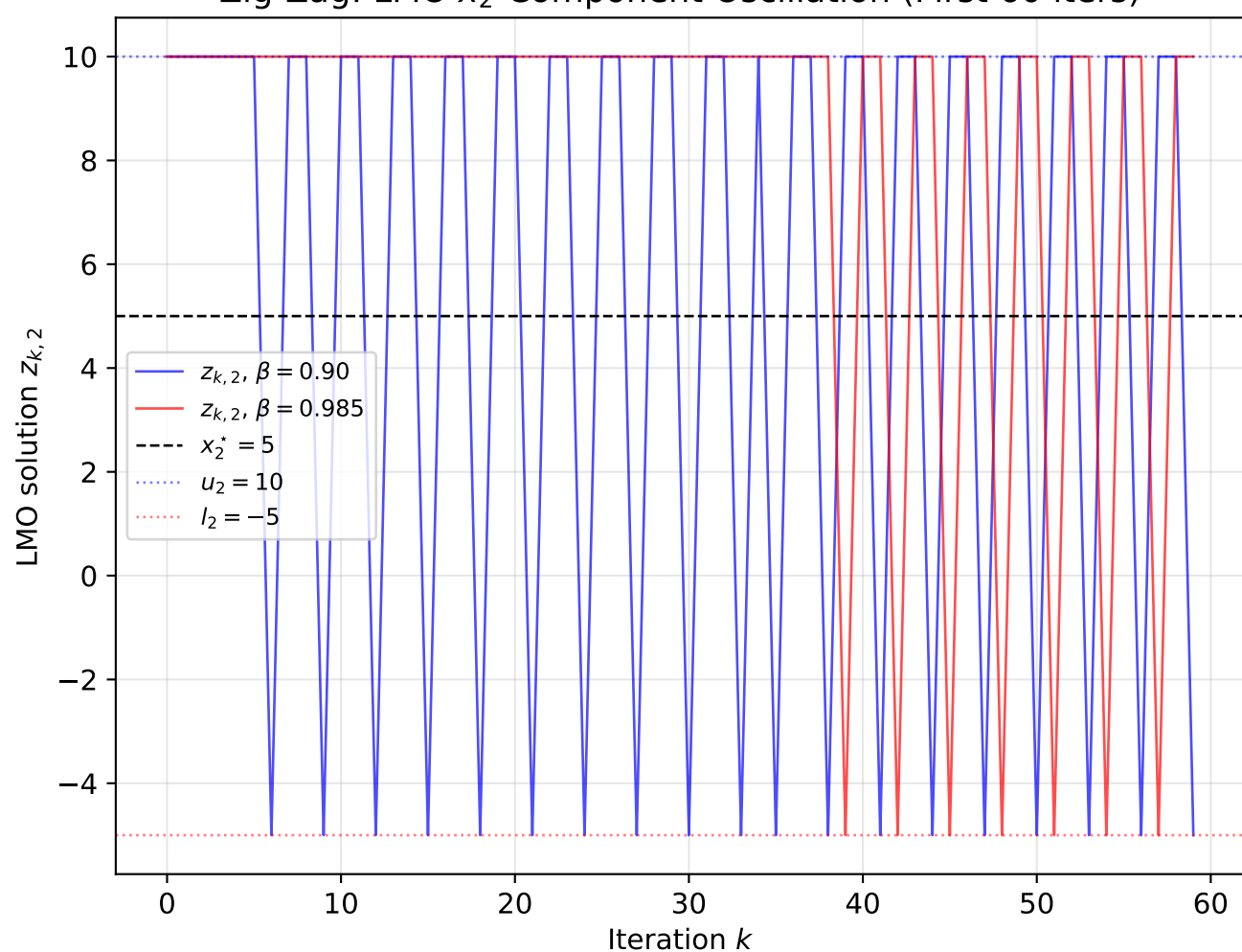
Zig-Zag: LMO x_2 -Component Oscillation (First 60 iters)
