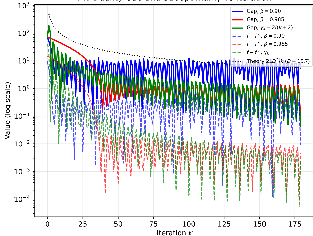
FW Duality Gap and Suboptimality vs Iteration
