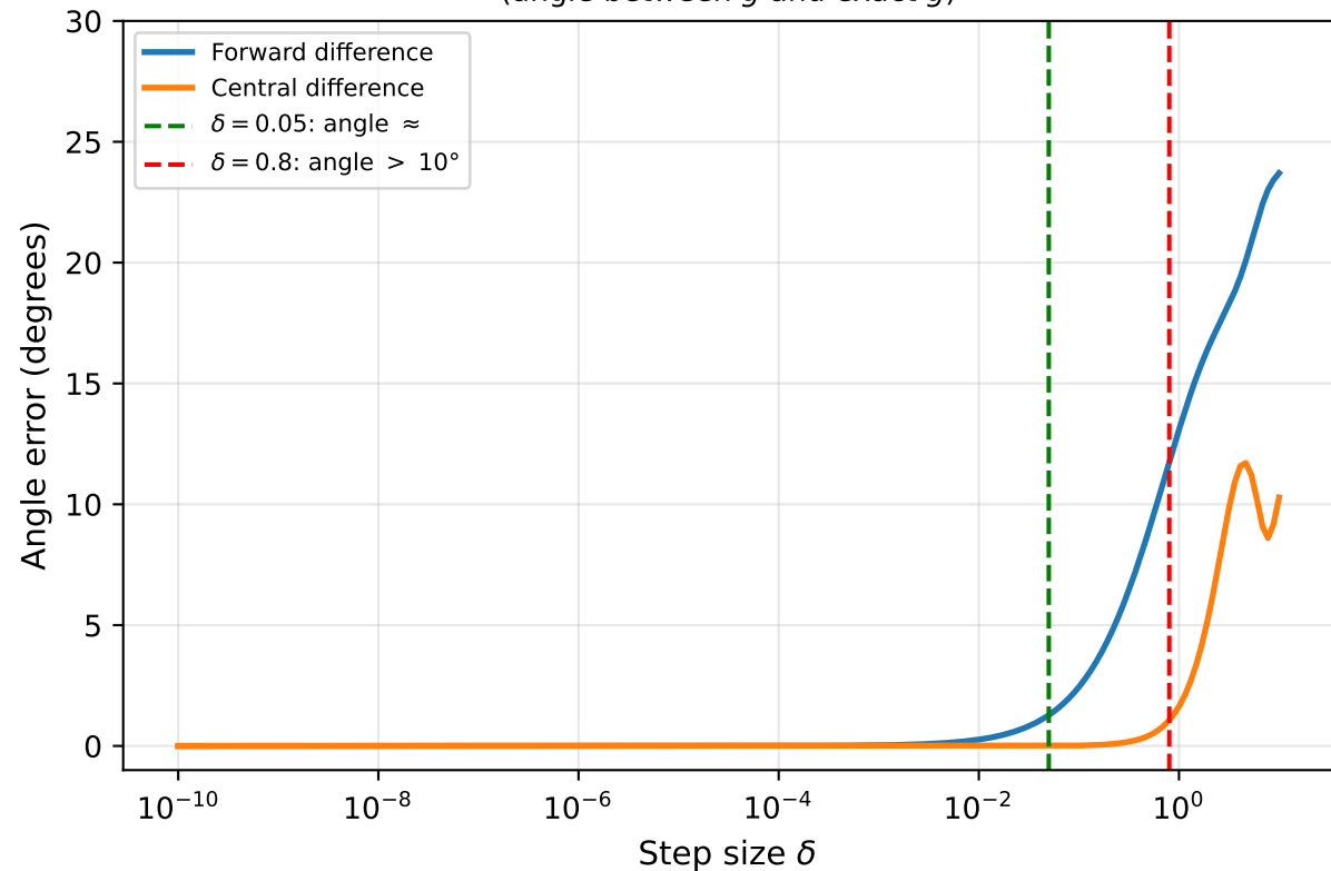
Gradient direction error vs \delta (angle between \hat{g} and exact g )
