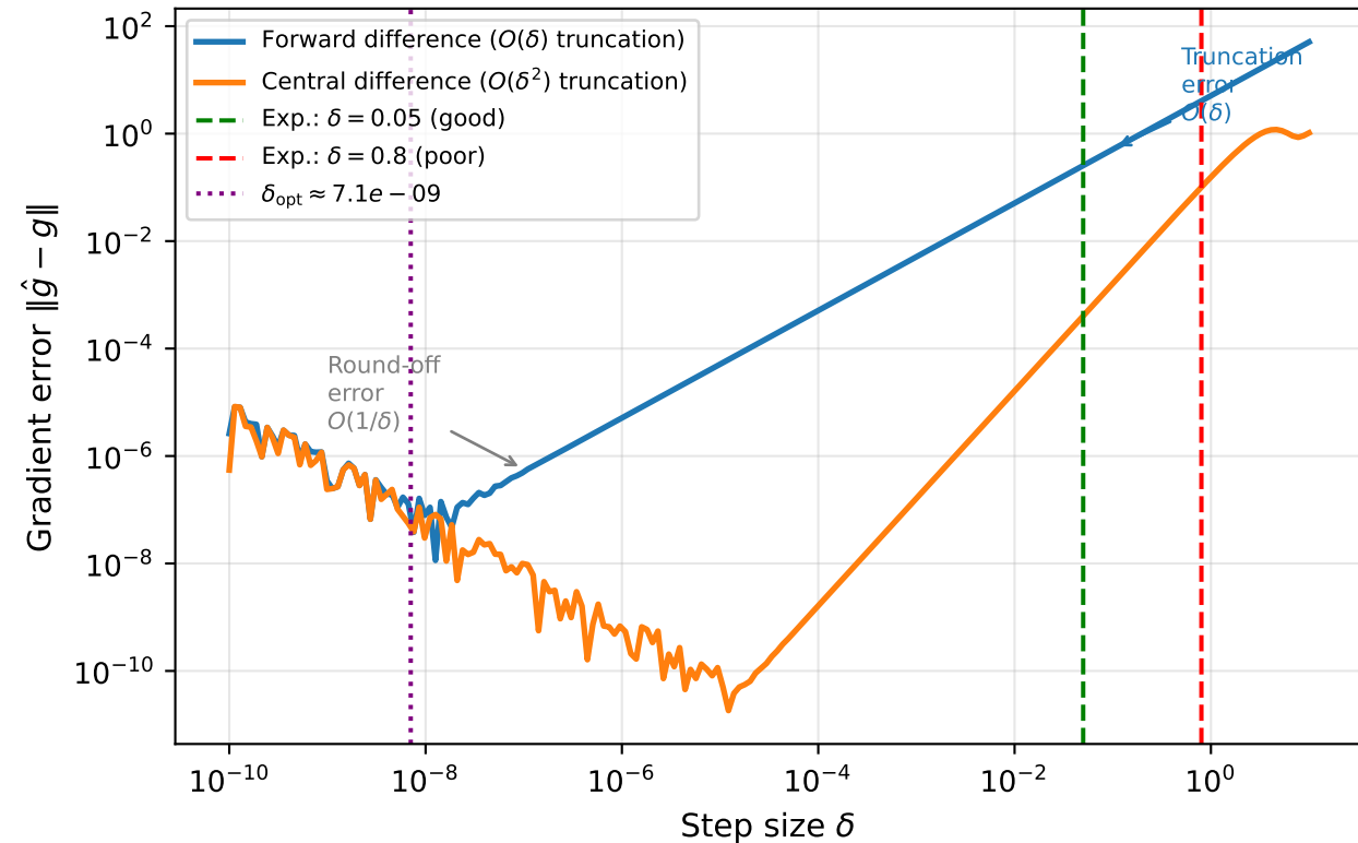
Gradient approximation error vs \delta (Benchmark B at x = (-0.2, 2.5) )
