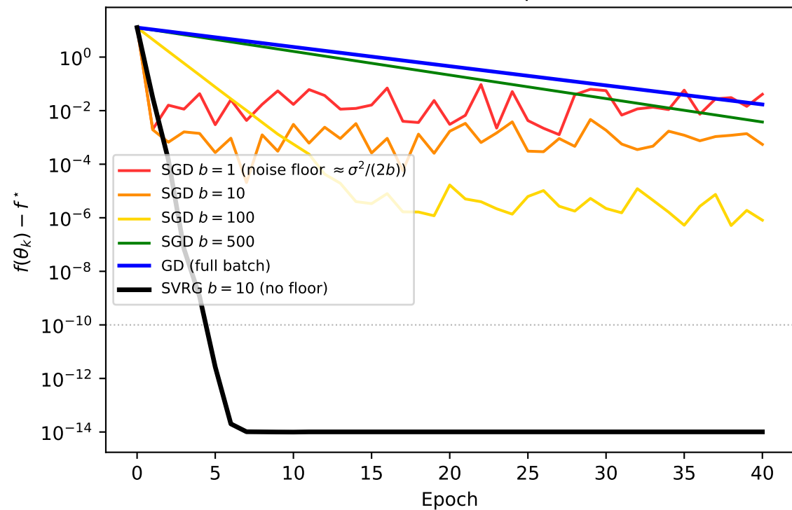
Mini-Batch SGD vs SVRG (Benchmark A, 40 epochs)
