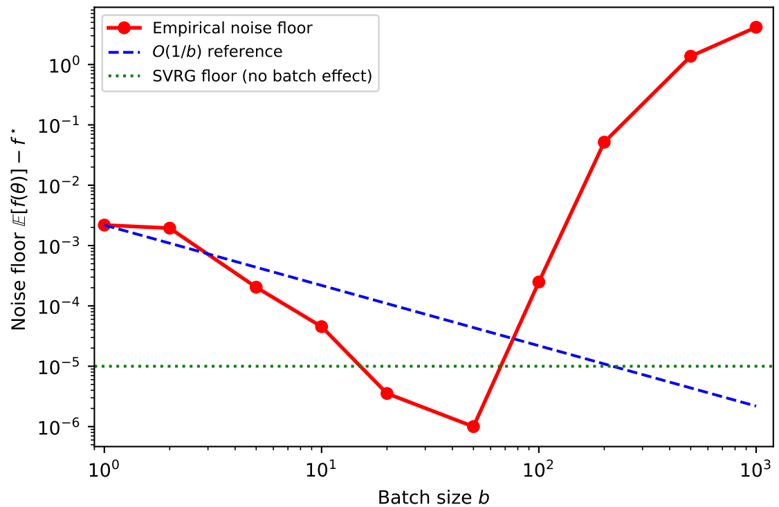
SGD Noise Floor vs Batch Size (Fixed \alpha = 0.01 , 60 epochs)
