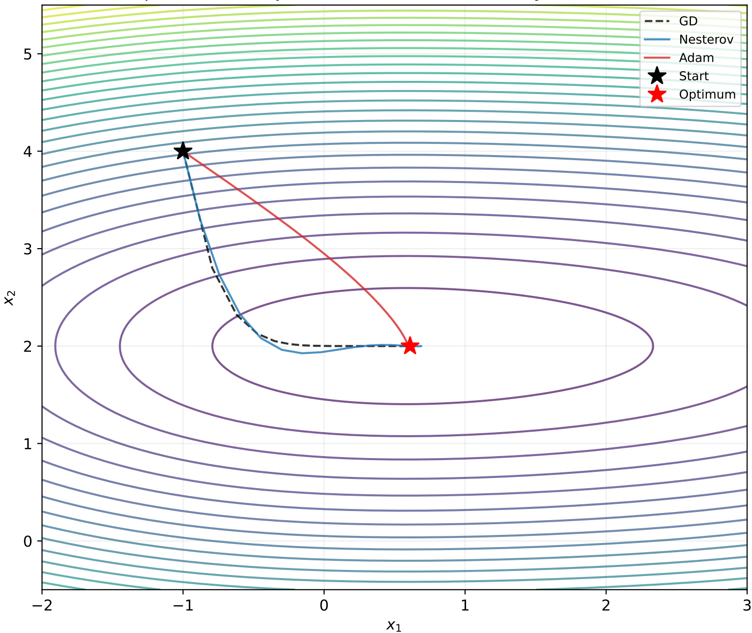
Q2: Optimisation Trajectories — Benchmark B (Toy Neural Network)
