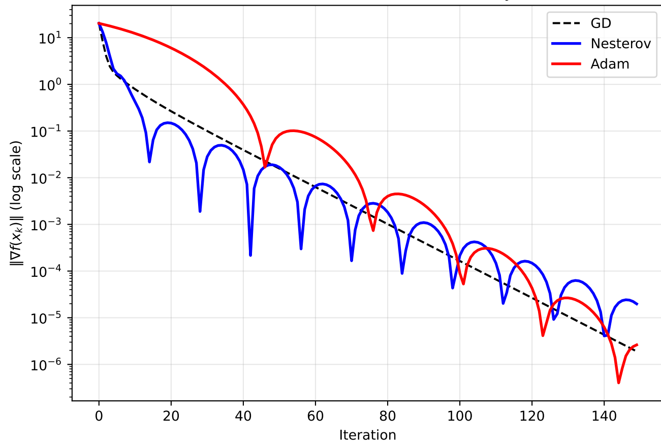
Q2: Gradient Norm — Benchmark B (Toy NN)
