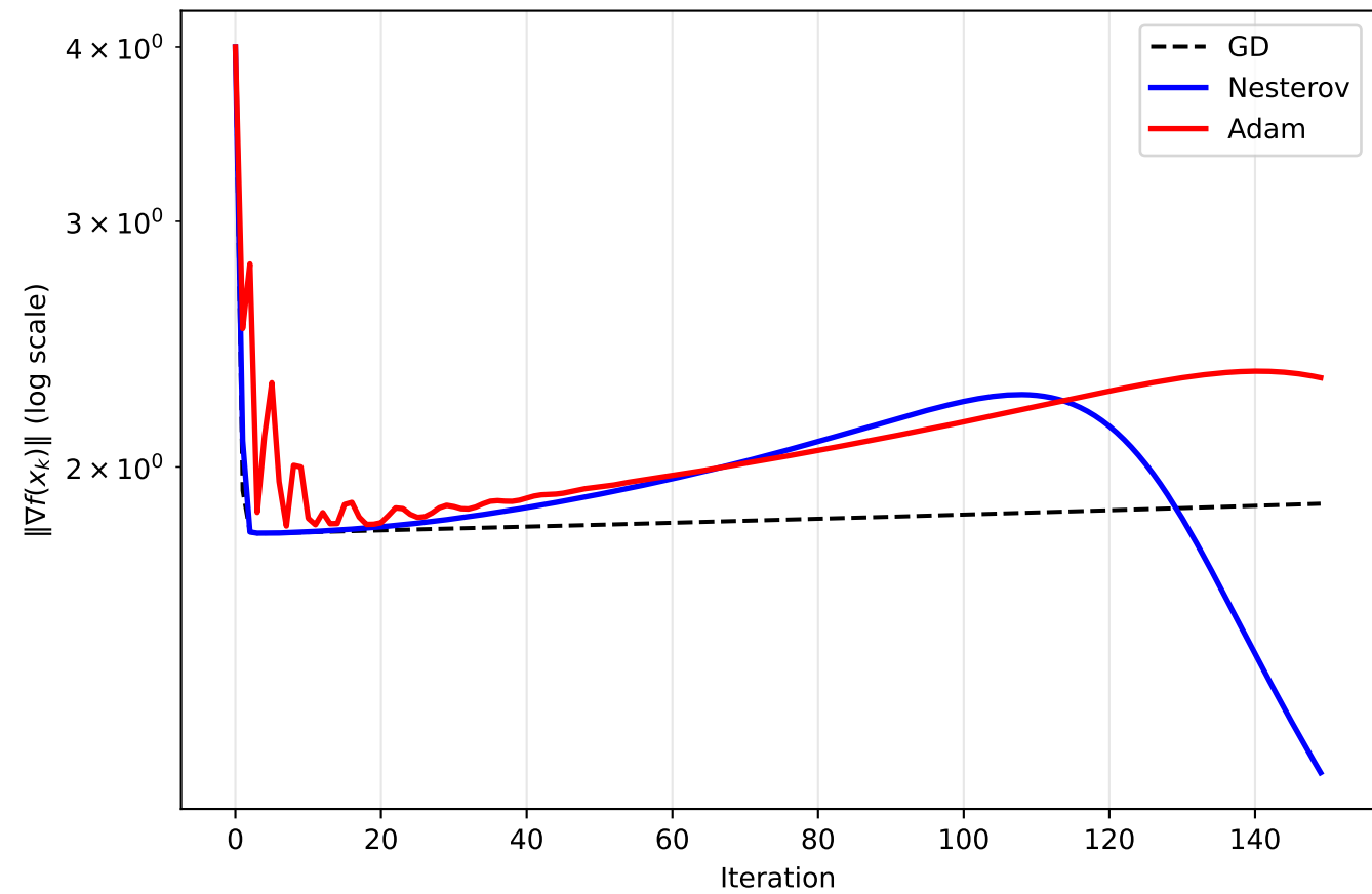
Q2: Gradient Norm — Benchmark C (Rosenbrock)
