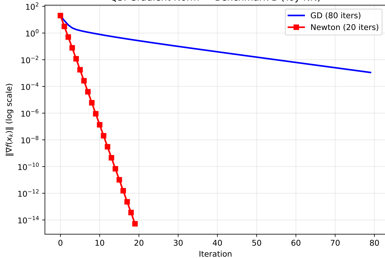
Q3: Gradient Norm — Benchmark B (Toy NN)
