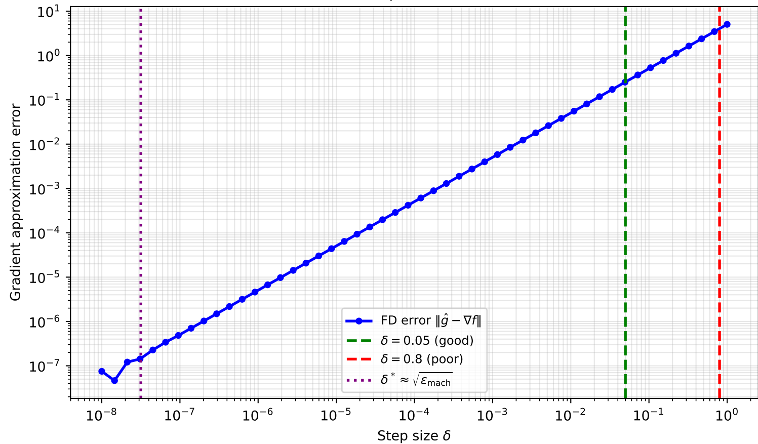
Q4: Finite Difference Error vs Step Size \delta (Benchmark B at x = (0.5, 1.5) )
