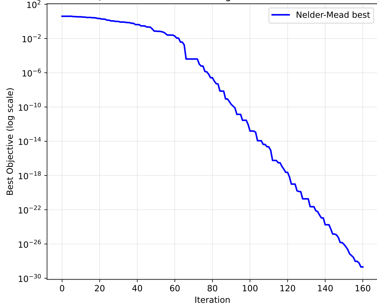
Q4B: Nelder-Mead Convergence — Rosenbrock
