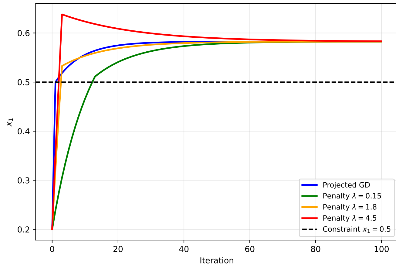
Q5: x_1 Trajectory — Constraint Enforcement
