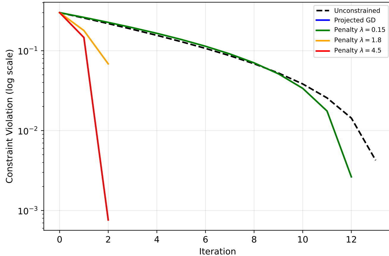
Q5: Constraint Violation \max(0, 0.5 - x_1)
