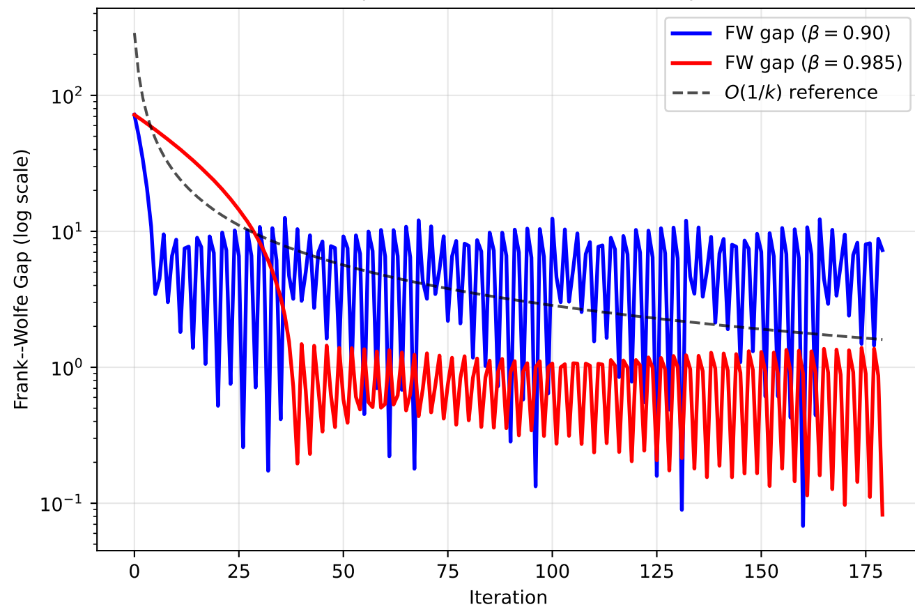
Q6: FW Gap \langle \nabla f(x_k), x_k - z_k \rangle — Interior Optimum
