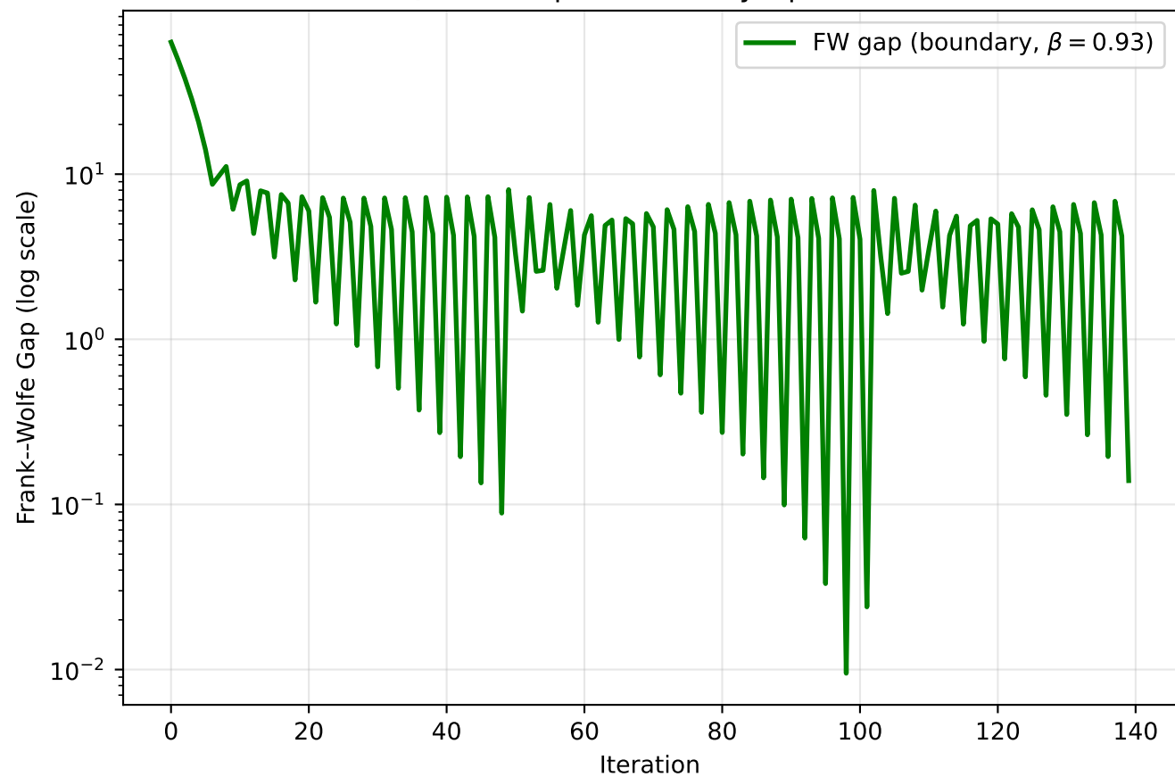
Q6: FW Gap — Boundary Optimum
