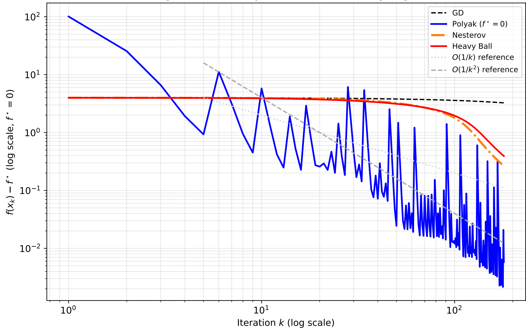
Convergence Rate Analysis on Rosenbrock (log--log scale)
