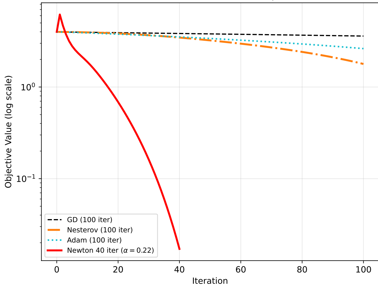
Rosenbrock: Best Methods Comparison
