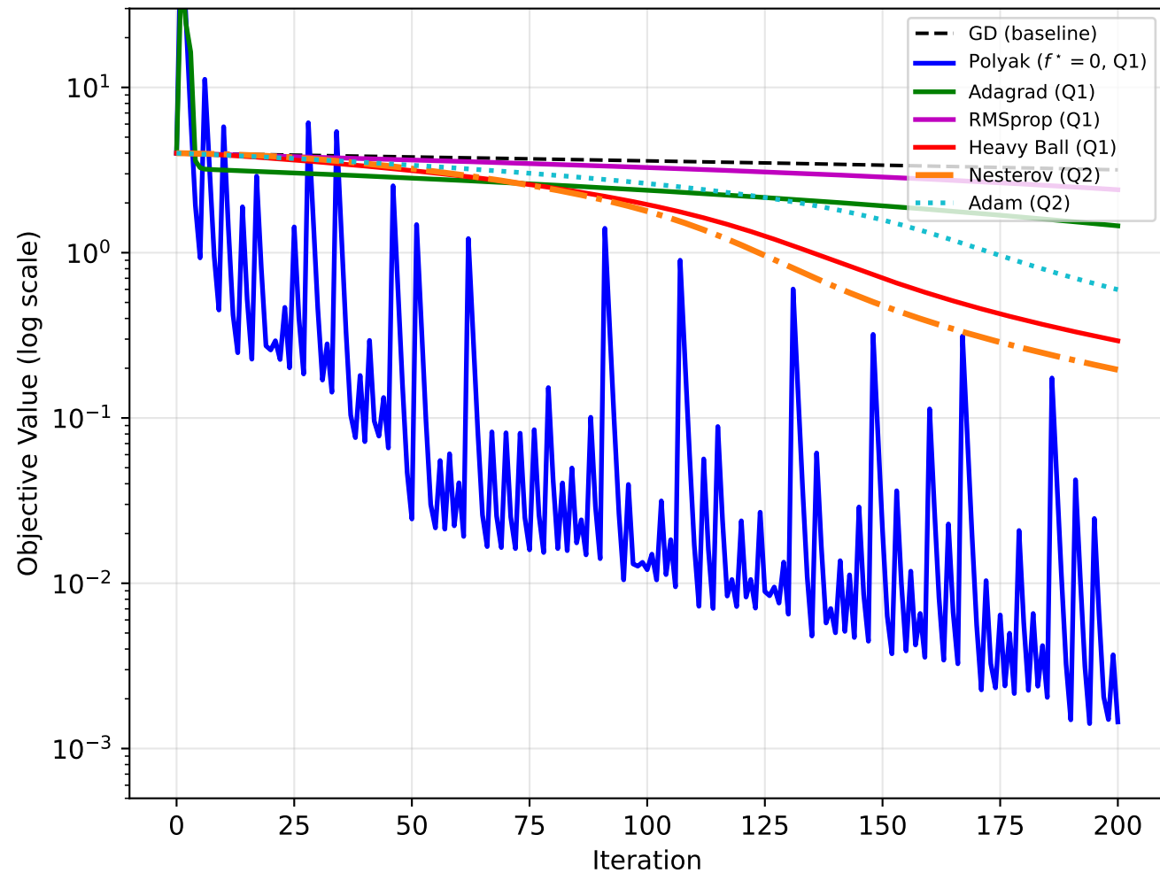
Rosenbrock: Q1 + Q2 Methods vs Iteration
