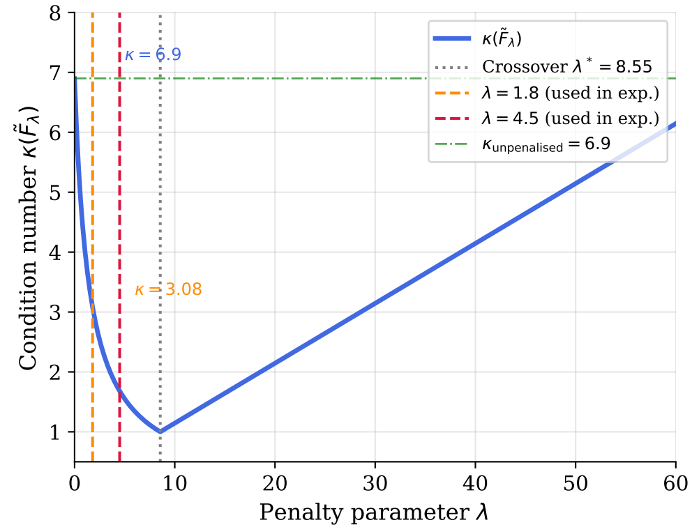
Penalised Condition Number vs \lambda
