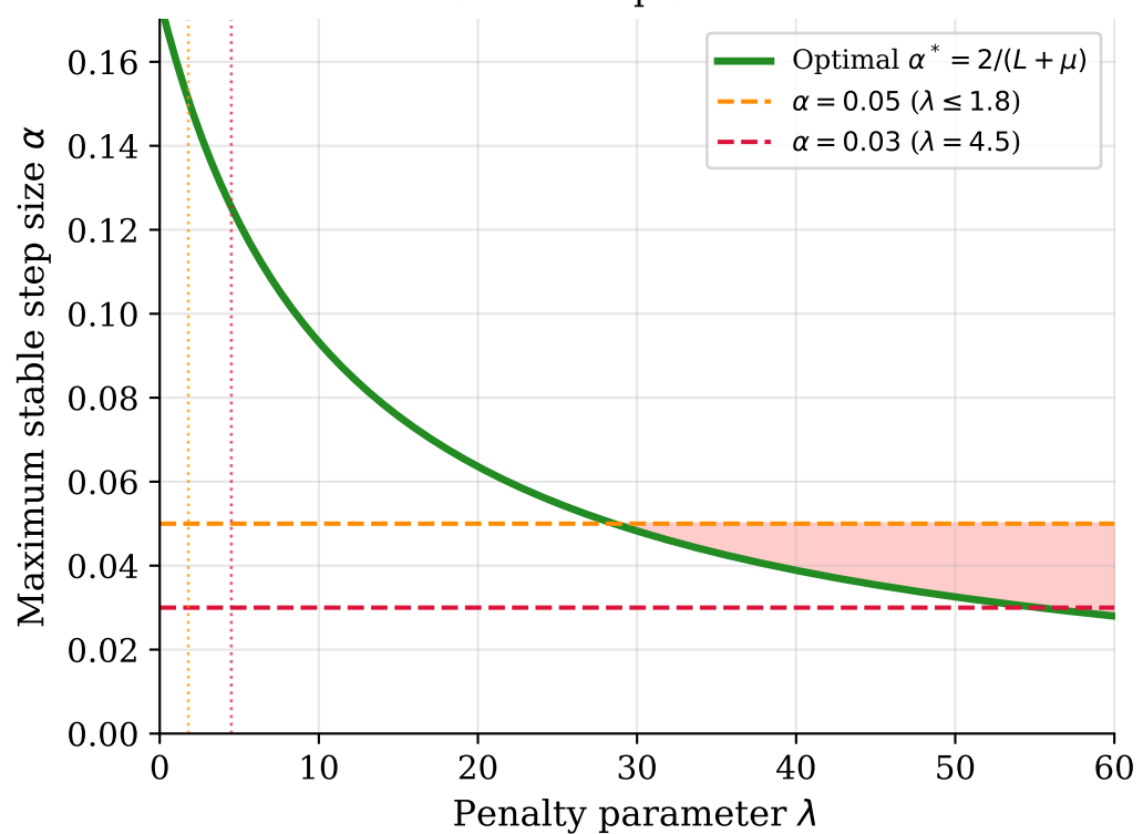
Stable Step Size vs \lambda
