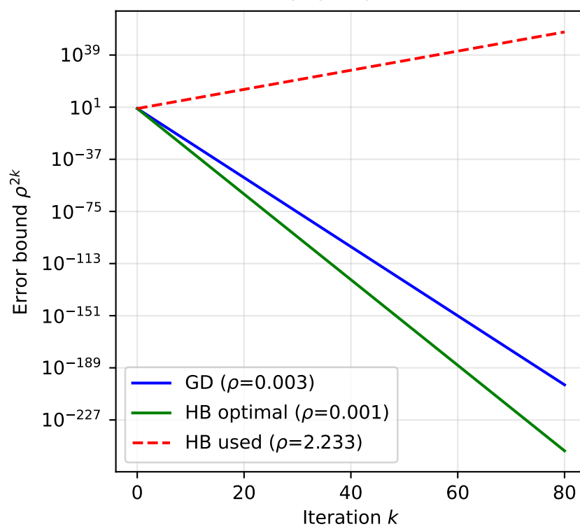
Heavy Ball vs GD Convergence Benchmark~A
