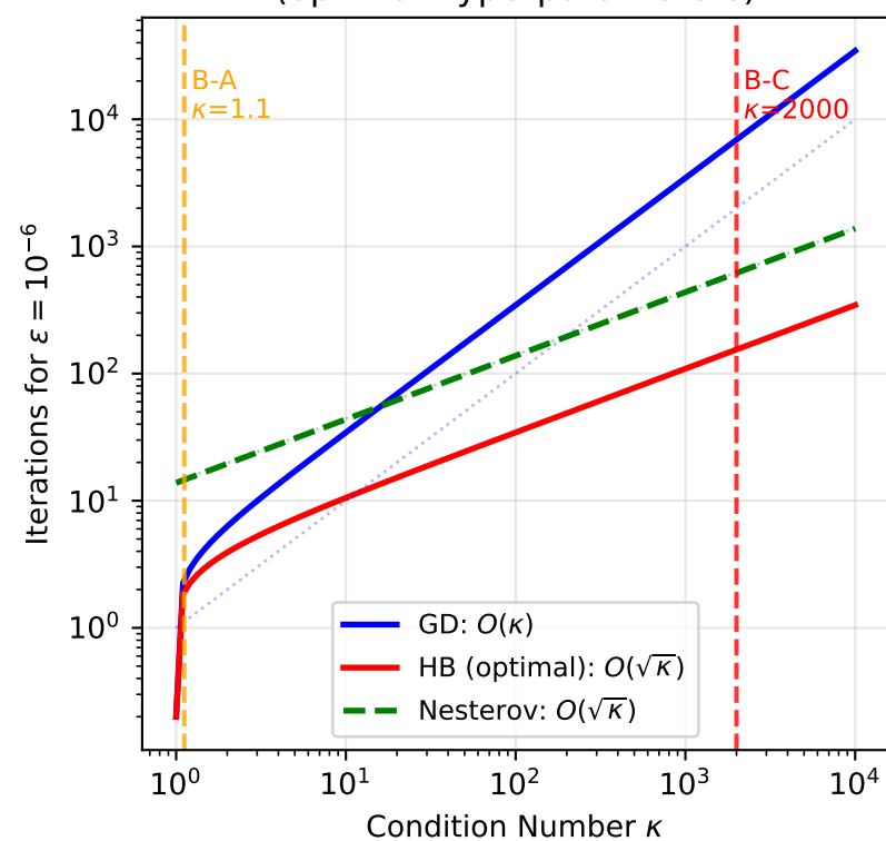
Algorithm Complexity Comparison (optimal hyperparameters)
