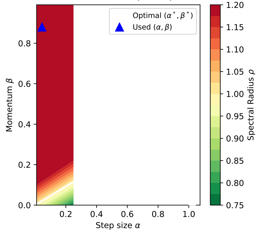
Heavy Ball Spectral Radius Benchmark~A ( \kappa=1.1 )
