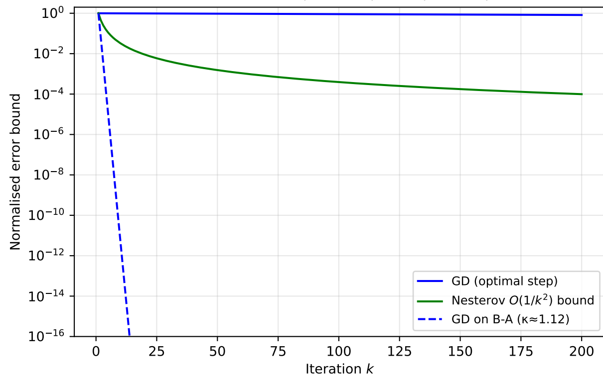
Convergence Rate Comparison Benchmark C ( \kappa=2000 ) vs A ( \kappa \approx 1.12 )
