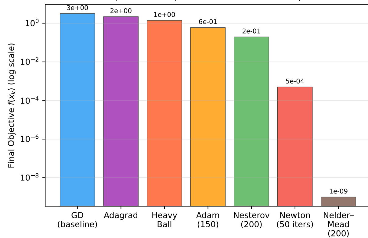
Final Objective on Rosenbrock (All Methods, Various Iteration Counts)
