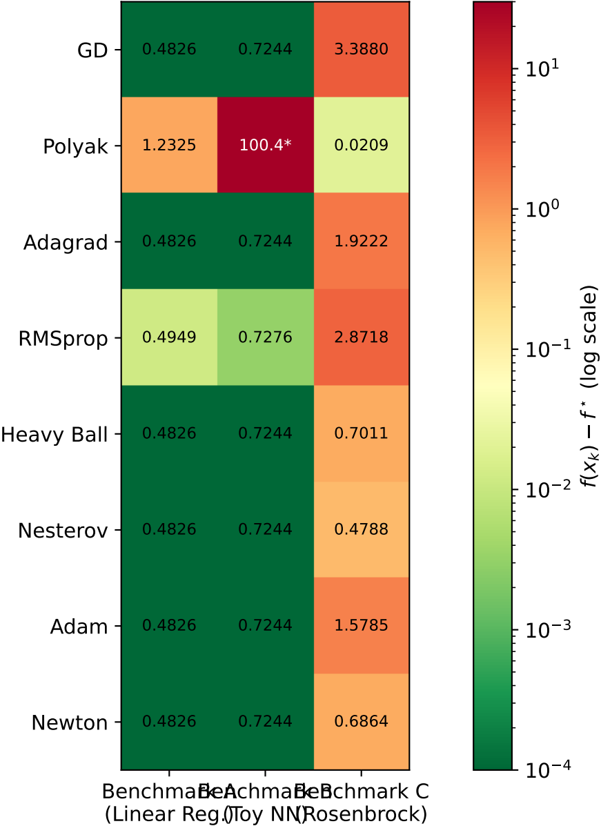
Performance Heatmap: Final Excess Objective f(x_k) - f^* (green = best, red = worst; log scale)
