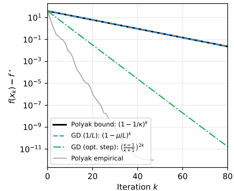
Convergence Rate: \kappa = 11.2
