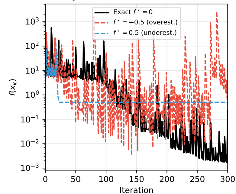
Polyak on Rosenbrock ( \kappa \approx 2508 )
