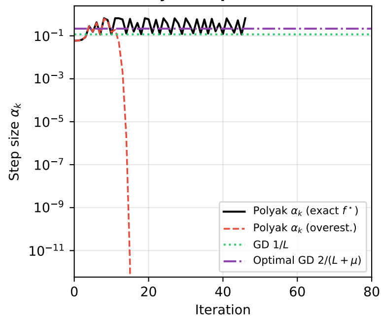
Polyak Step Evolution
