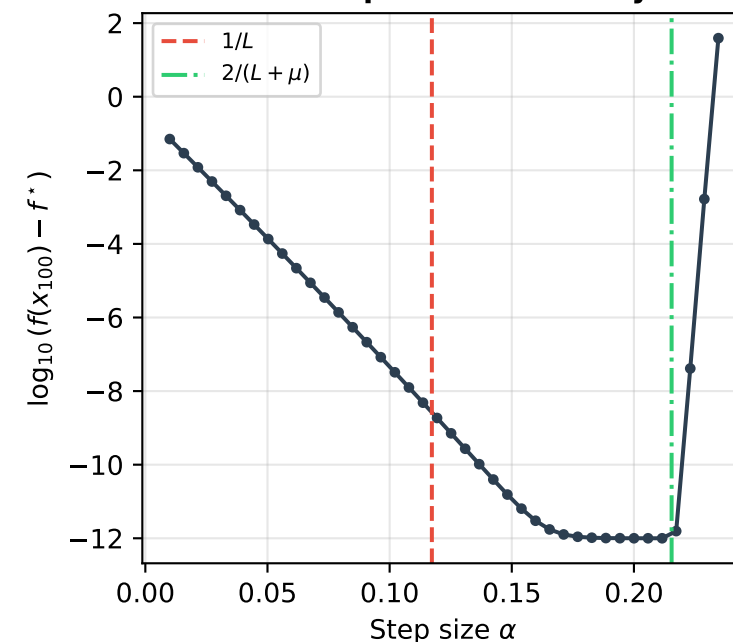
GD: Step-Size Sensitivity
