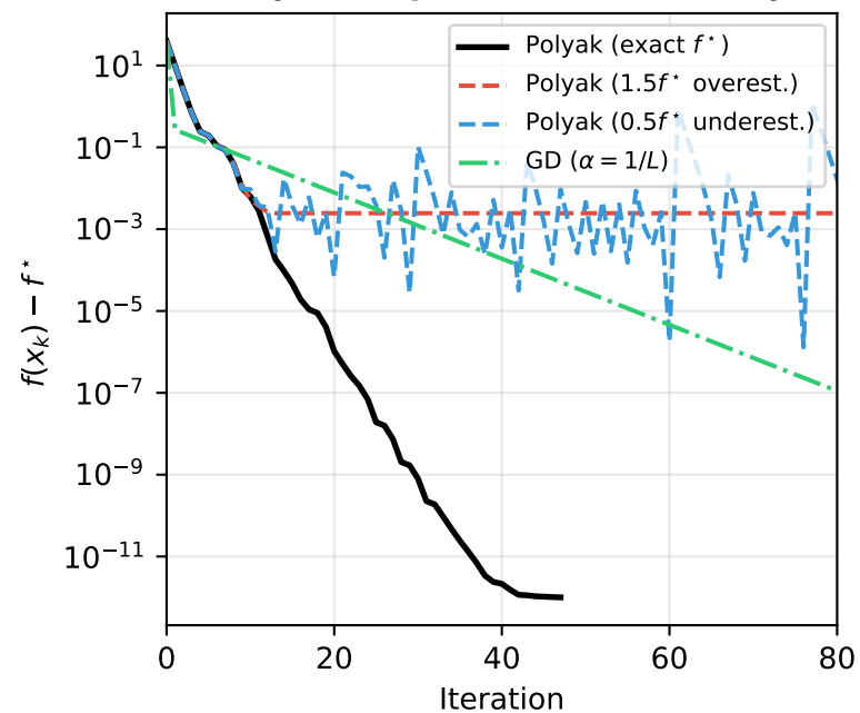
Polyak Step Size: f^* Sensitivity
