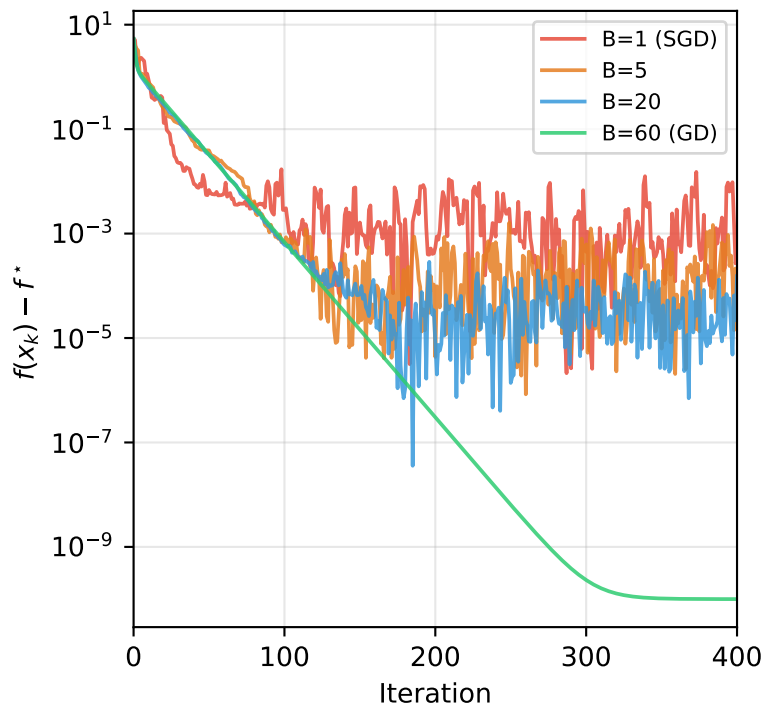
SGD: Batch Size Effect
