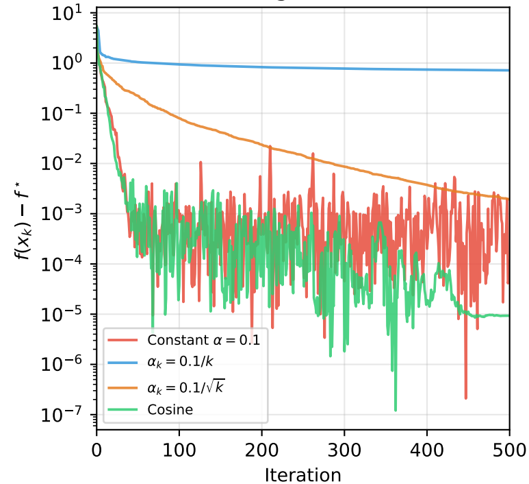
SGD Learning Rate Schedules
