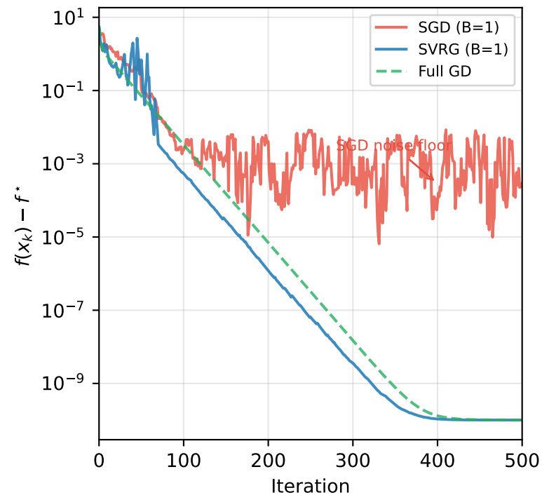
SGD vs SVRG
