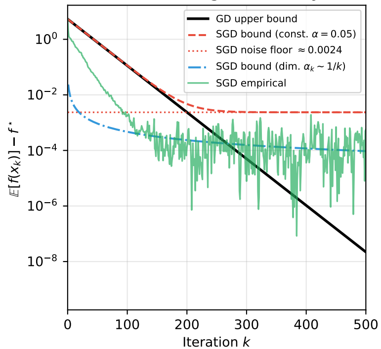
SGD Convergence Theory
