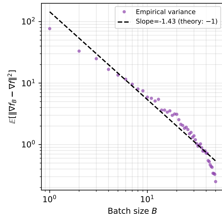
Gradient Variance \propto 1/B
