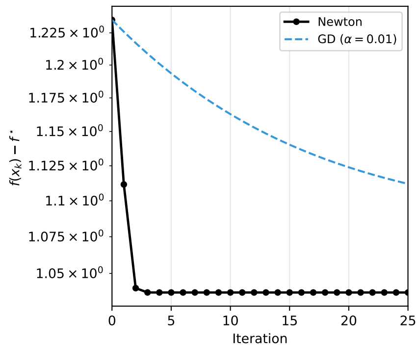
Newton vs GD: Benchmark B
