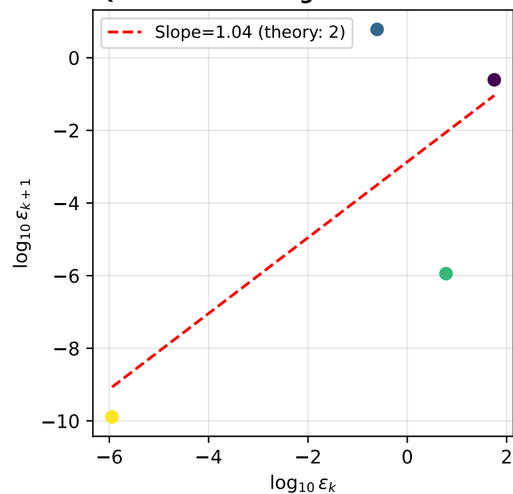
Quadratic Convergence Verification
