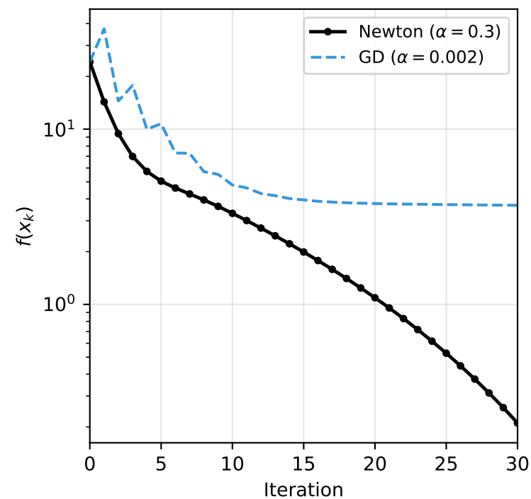
Newton vs GD: Rosenbrock ( \kappa \approx 2508 )
