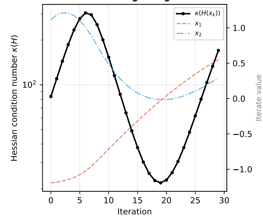
Hessian Conditioning Along Newton Path
