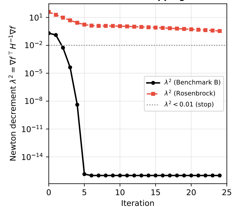
Newton Decrement Stopping Criterion
