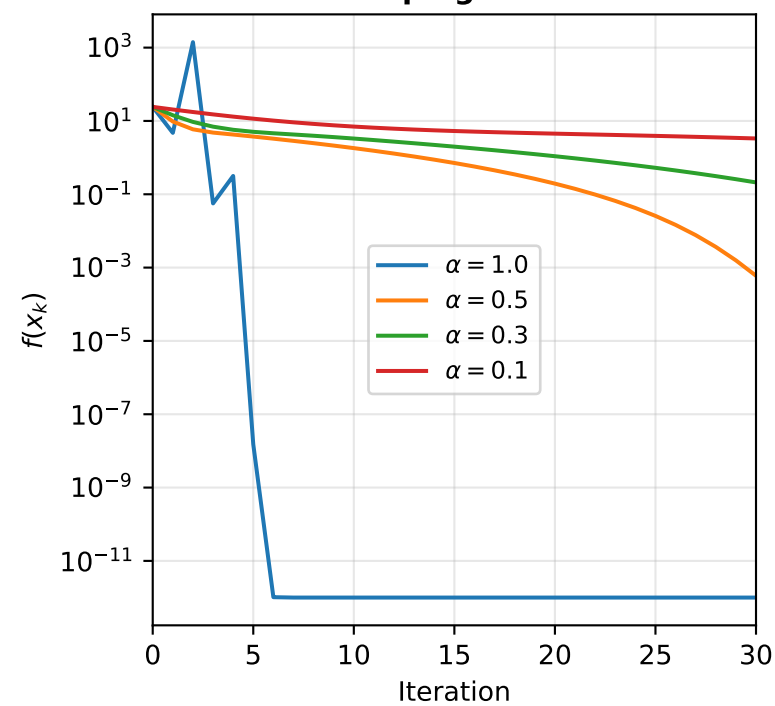
Newton: Damping on Rosenbrock
