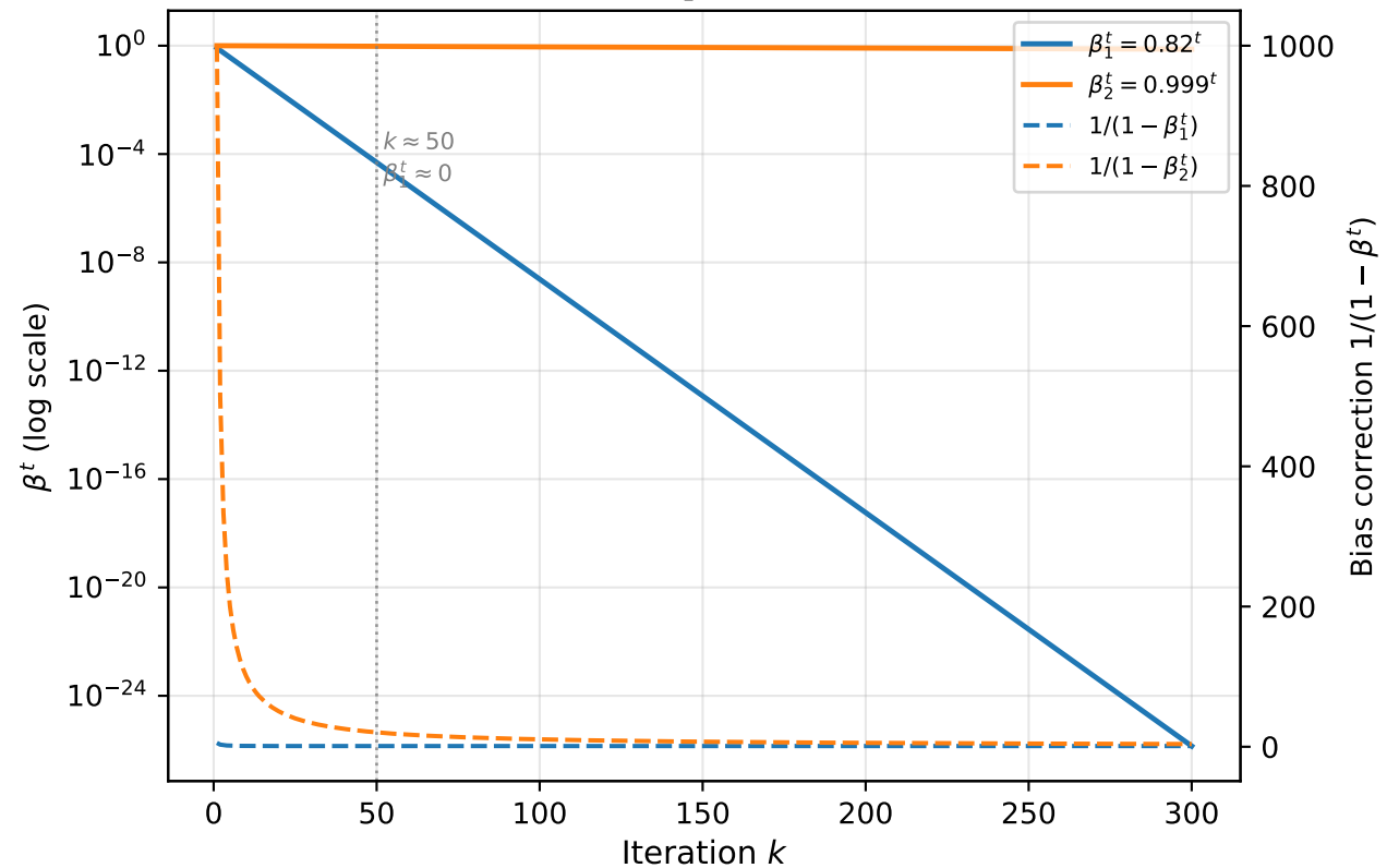
Bias Correction Decay: \beta_1^t Negligible after \sim 50 steps
