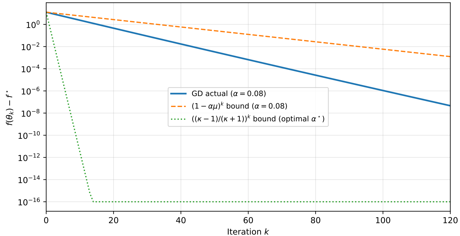
GD Convergence: Benchmark A ( \kappa \approx 1.12 , actual vs. bounds)
