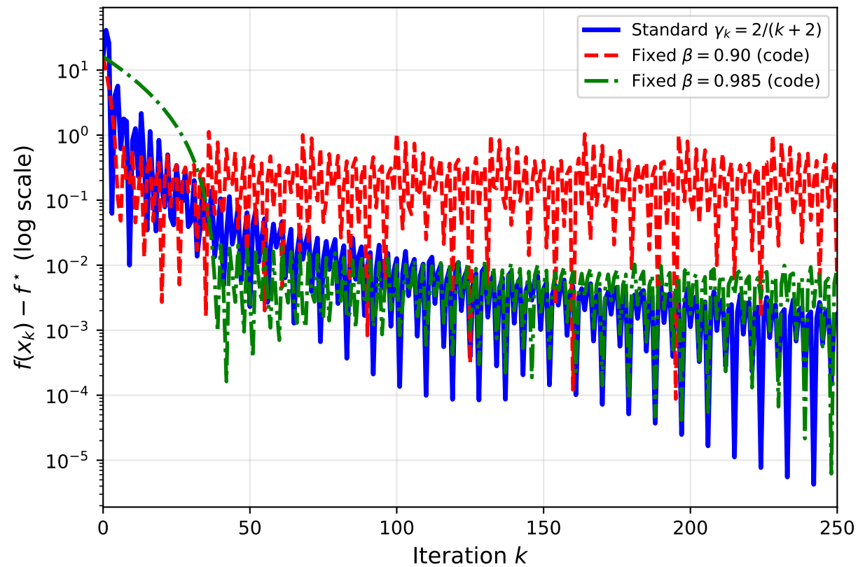
Interior Optimum ( f^* = 0 at (1, 5) )
