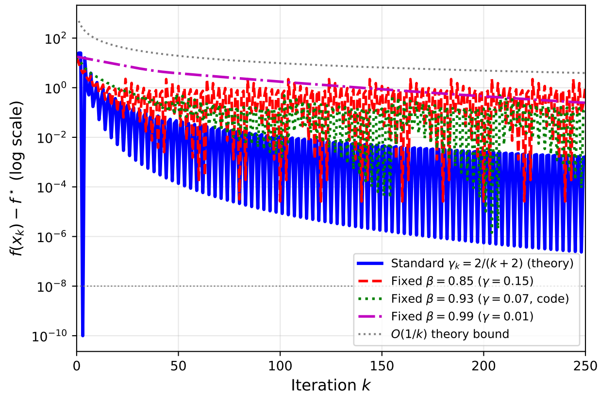
Boundary Optimum ( f^* = 0.25 at (0.5, 0) )
