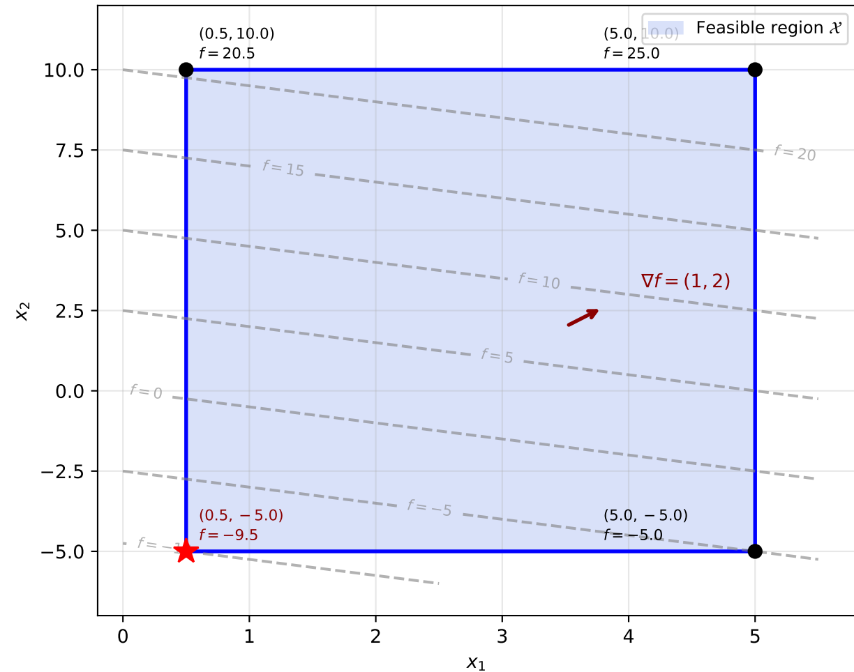
LP over Box: Optimal at Vertex (0.5, -5)
