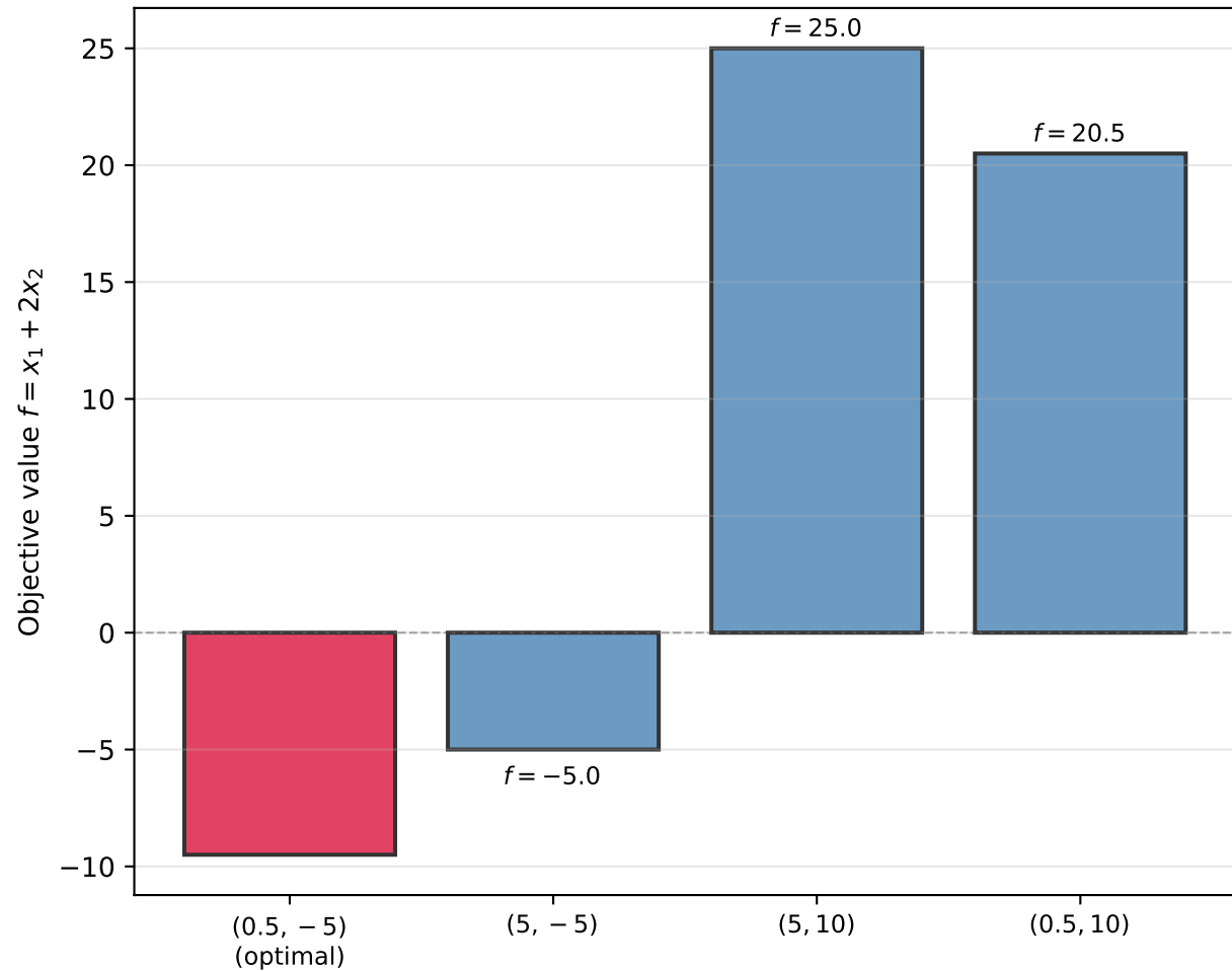
LP Objective at All 4 Vertices of \mathcal{X}
