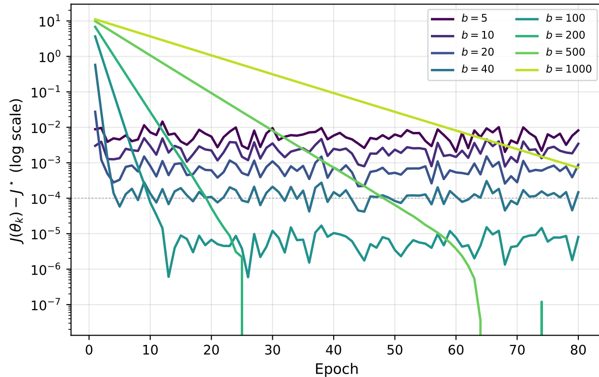
Mini-batch SGD: Convergence vs Batch Size ( \alpha = 0.06 , 80 epochs)
