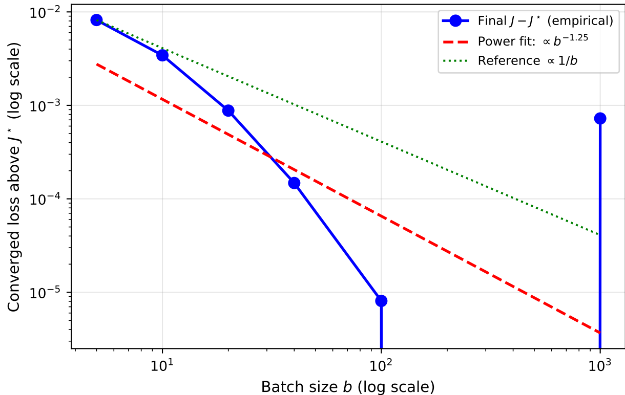
Noise Floor vs Batch Size (fitted slope = -1.25 \approx -1 , confirming O(1/b) )
