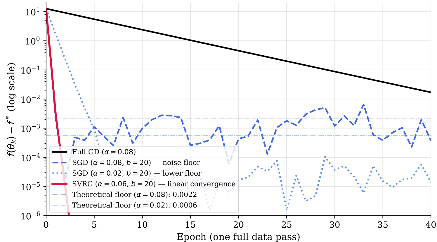
SGD vs SVRG: Variance Reduction Effect on Benchmark A (Linear convergence vs irreducible noise floor)
