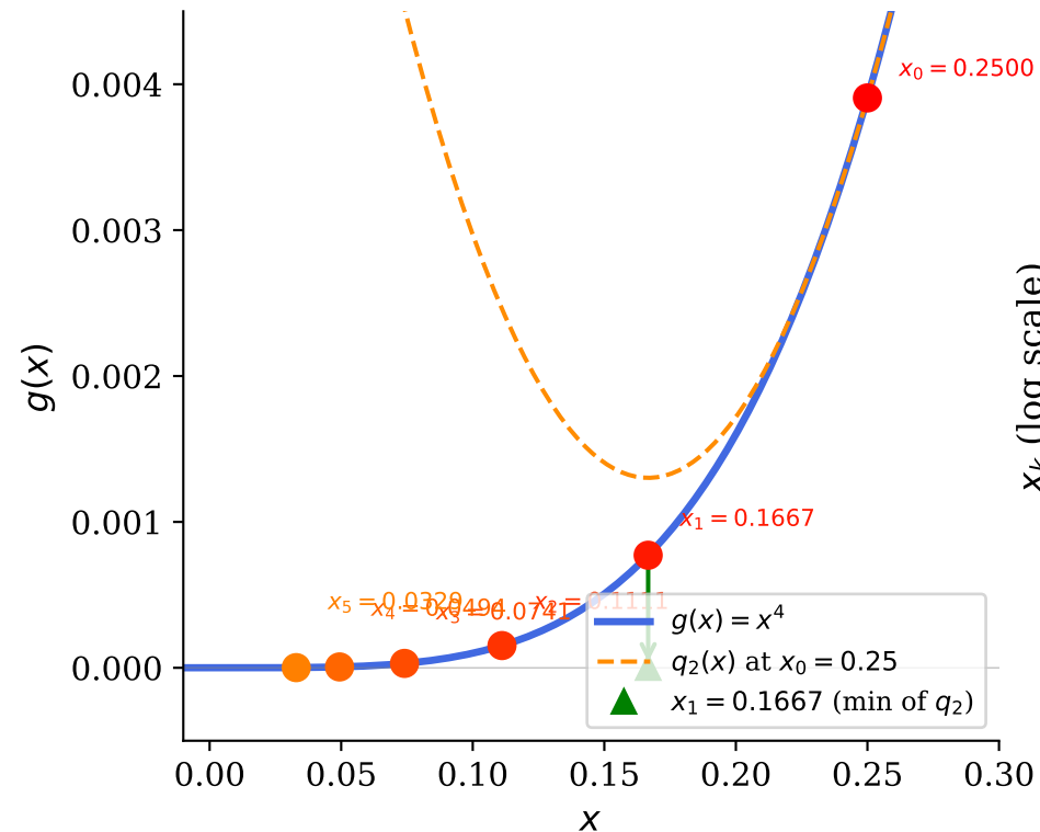
Newton Iterates on g(x) = x^4
