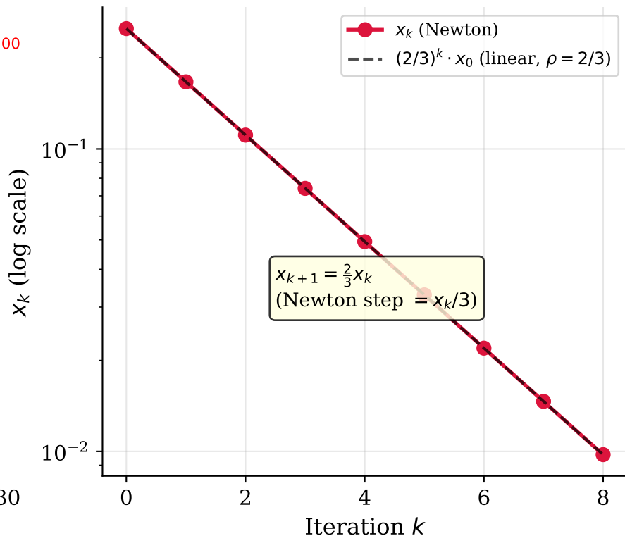
Linear (not quadratic) convergence: g'(x^*) = 0 at x^* = 0 (degenerate Hessian)
