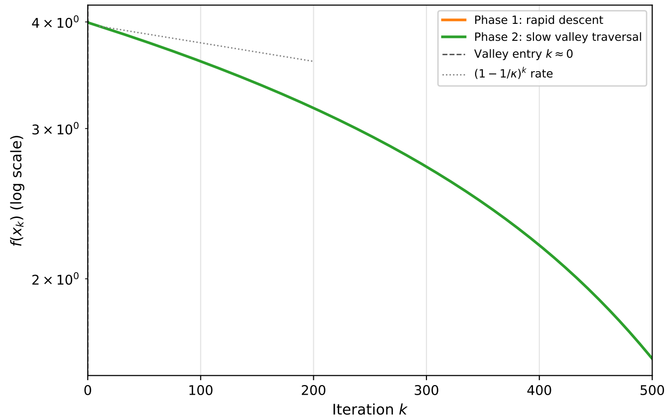
GD on Rosenbrock: convergence phases (Phase 1 fast, Phase 2 slow)
