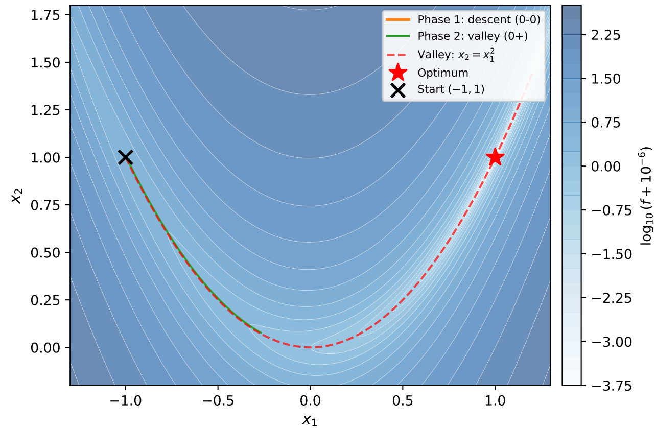
GD on Rosenbrock: two phases (500 iterations, \alpha = 0.0012 )
