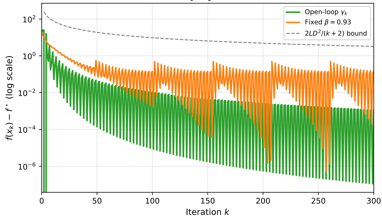
Boundary optimum: convergence comparison
