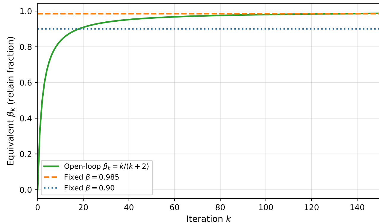
Step size (retain fraction) comparison
