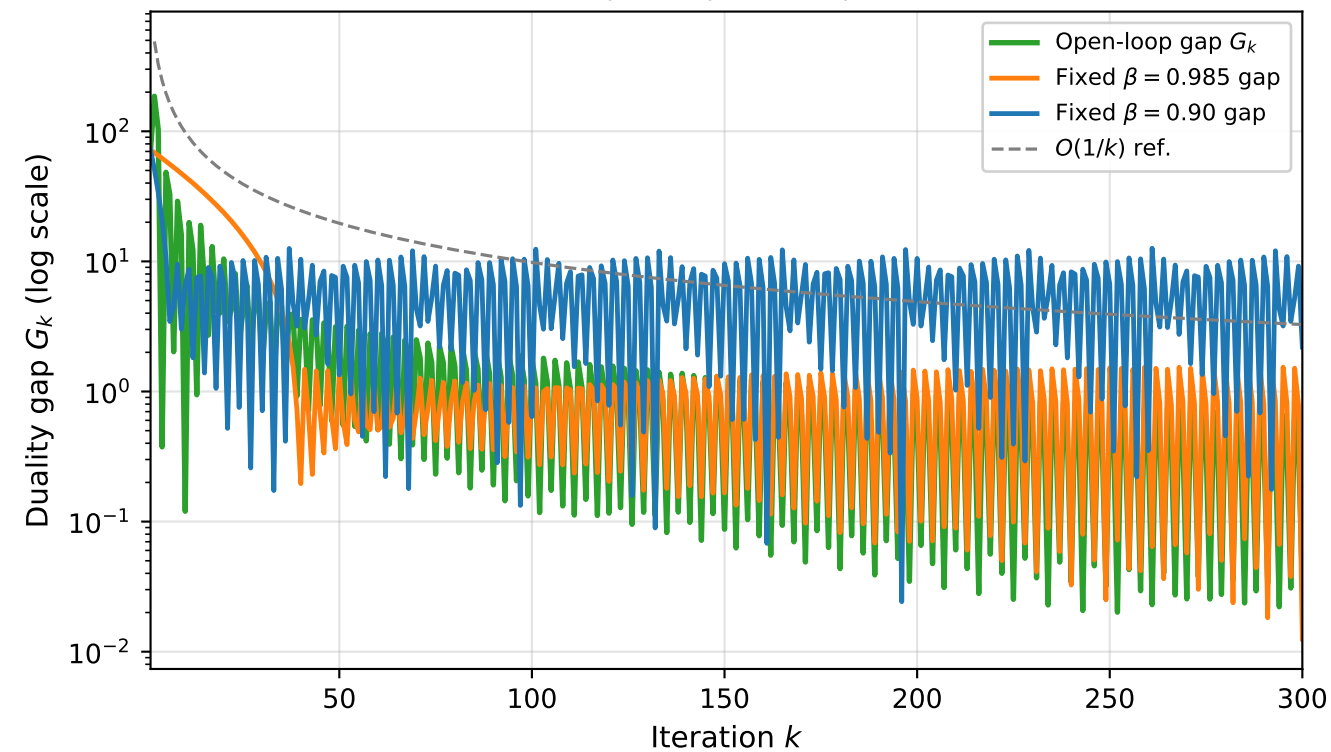
Step size (retain fraction) comparison
