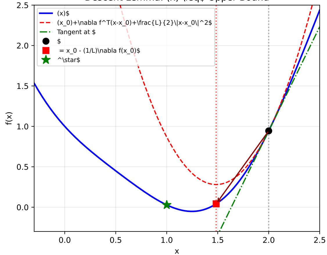
Descent Lemma: f(x) \leq Upper Bound
