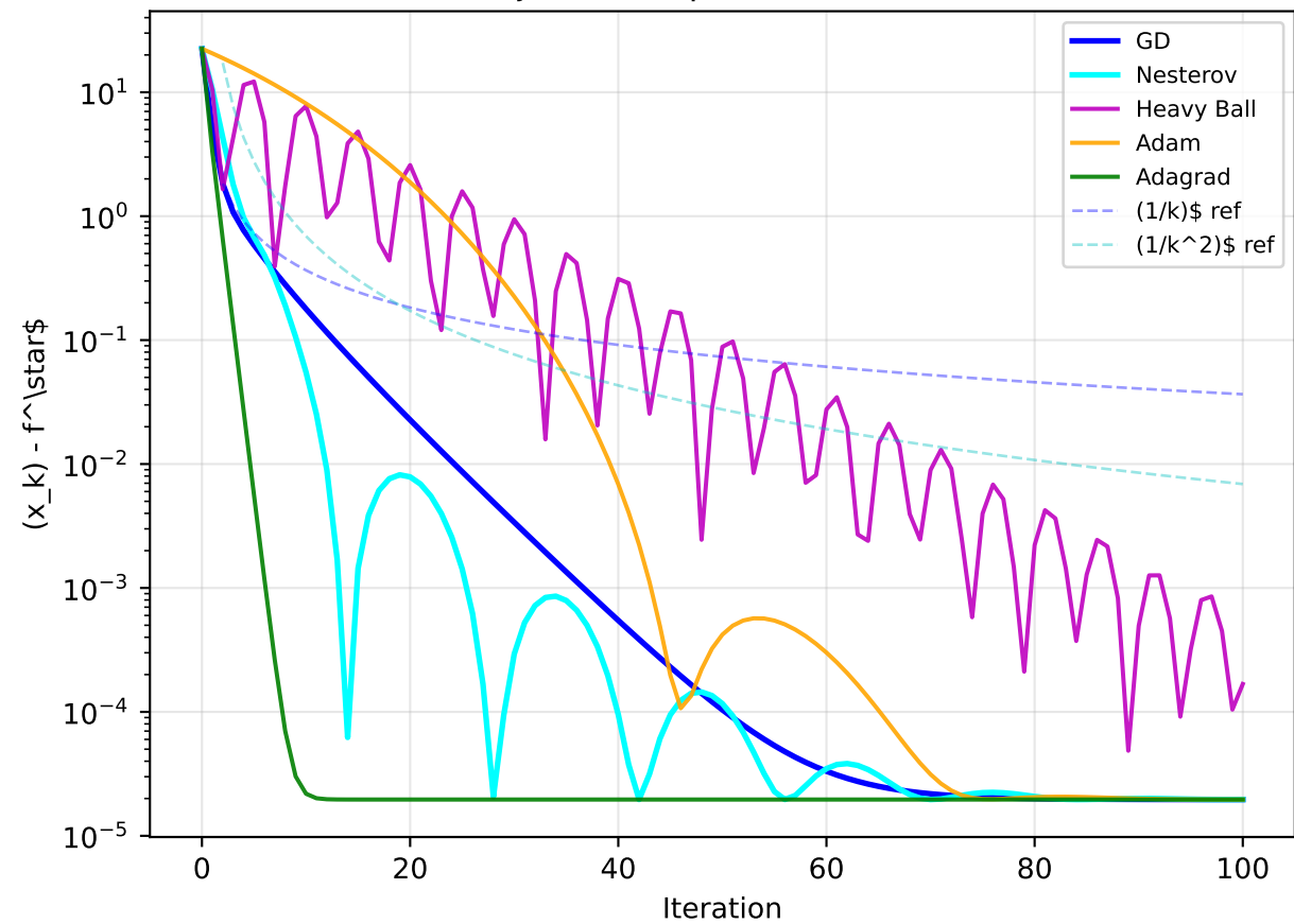
Objective Gap (Benchmark B)
