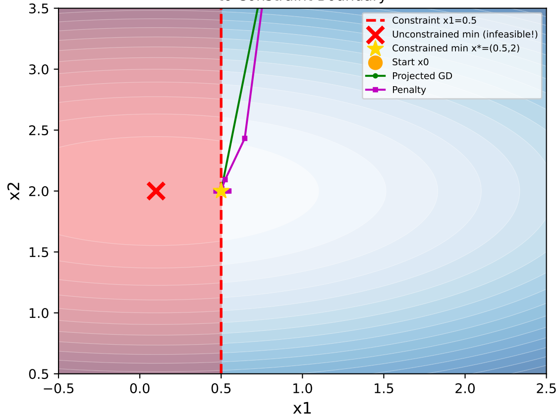
Active Constraint: Methods Converge to Constraint Boundary
