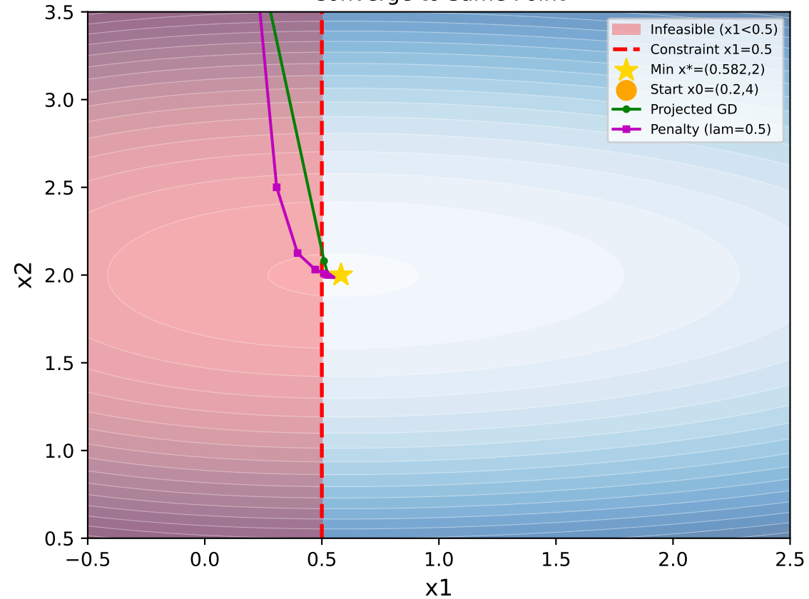
Inactive Constraint: All Methods Converge to Same Point
