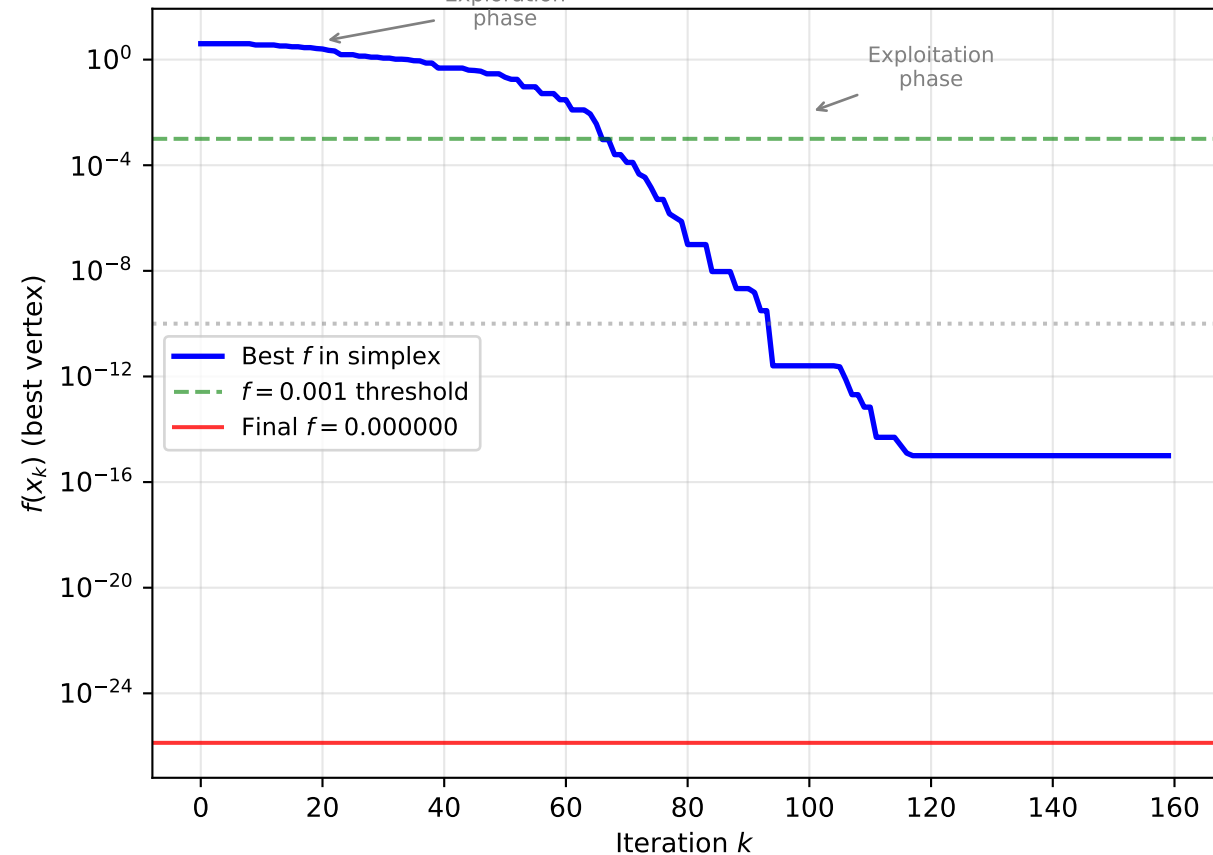
Nelder--Mead Convergence Final: f = 0.000000 at (1, 1) in 160 iters
