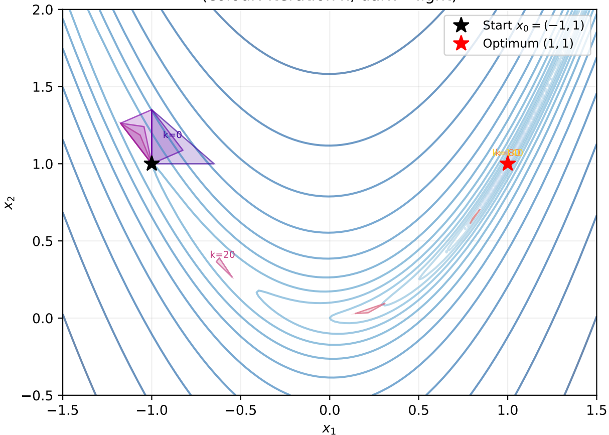
Nelder--Mead Simplex Evolution (colour: iteration k , dark \rightarrow light)
