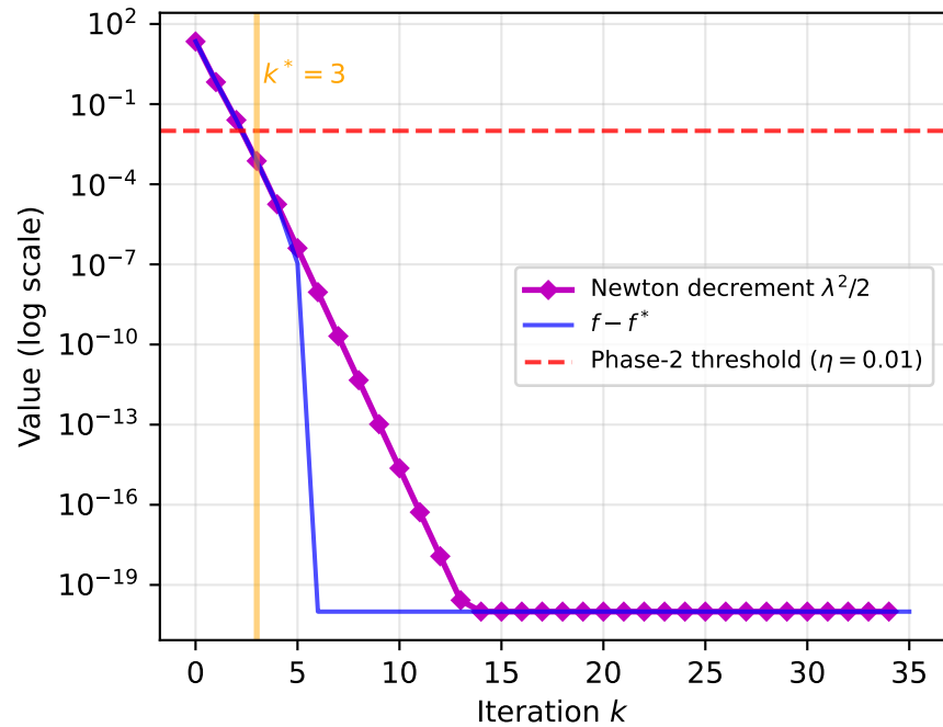
Newton Decrement Certificate \lambda^2/2 \geq f - f^* (self-concordant)
