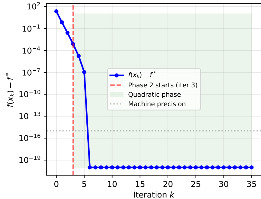
Newton Two-Phase Convergence (Benchmark~B)
