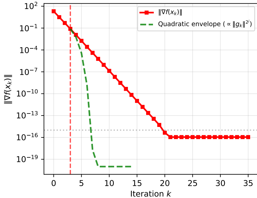
Gradient Norm: Linear \rightarrow Superlinear (Benchmark~B)
