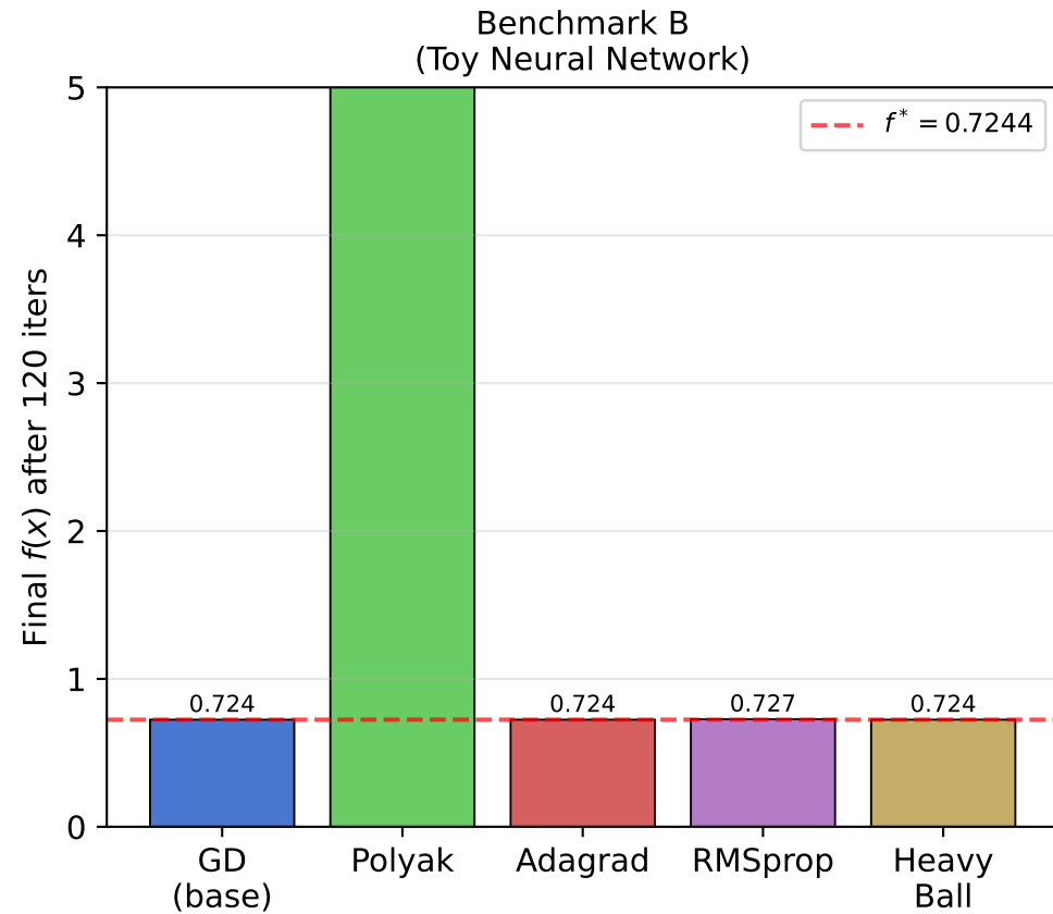
Q1: Final Objective Values — Adaptive Step-Size Methods (120 iterations)
