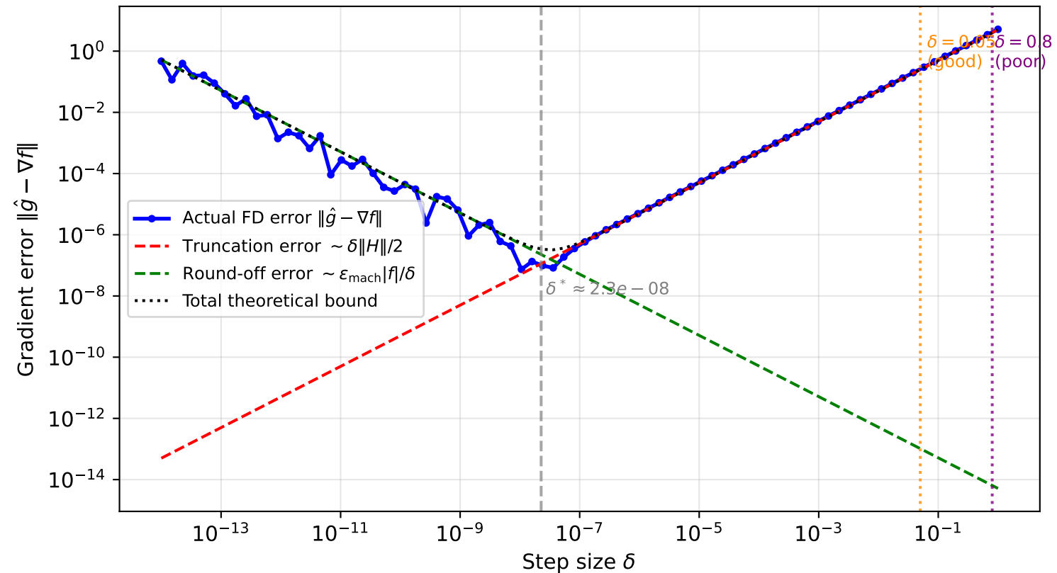
Q4: Forward Finite Difference Approximation Error vs Step Size \delta (Benchmark B at x_0 = (-1, 4) )
