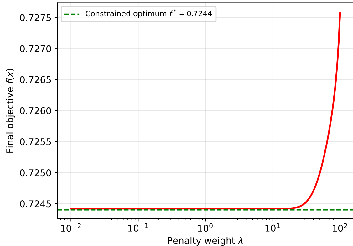
Final Objective vs Penalty Weight \lambda
