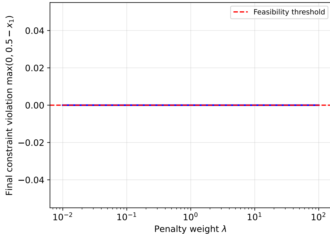
Constraint Violation vs Penalty Weight \lambda
